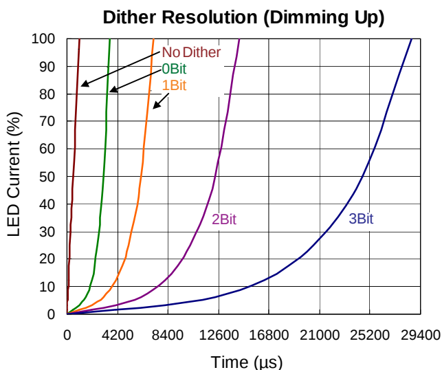
Figure 12. LED Current (Dimming Up) vs. Time
