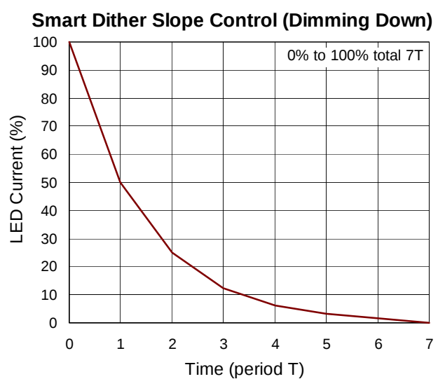
Figure 11. LED Current (Dimming Down) vs. Time
