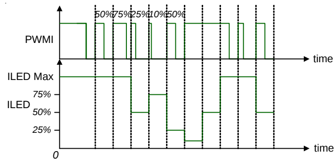
Figure 2. DC Dimming
