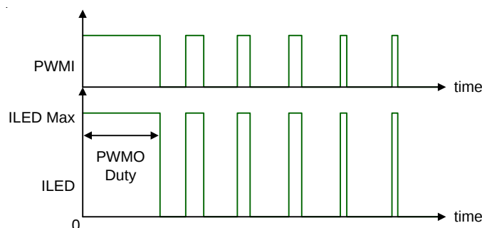
Figure 1. PWM Dimming
