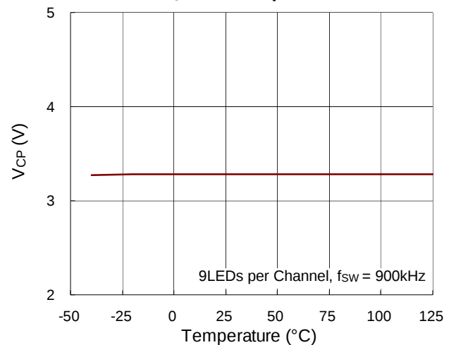
V_{CP} vs. Temperature
