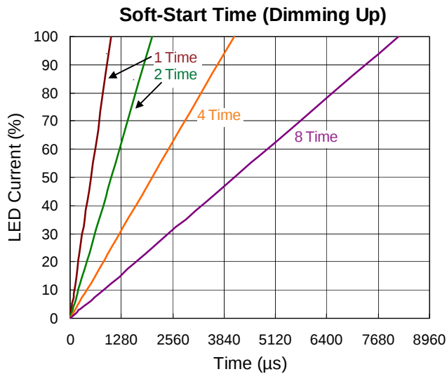
Figure 8. LED Current (Dimming Up) vs. Soft Start Time
