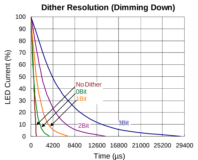
Figure 13. LED Current (Dimming Down) vs. Time
