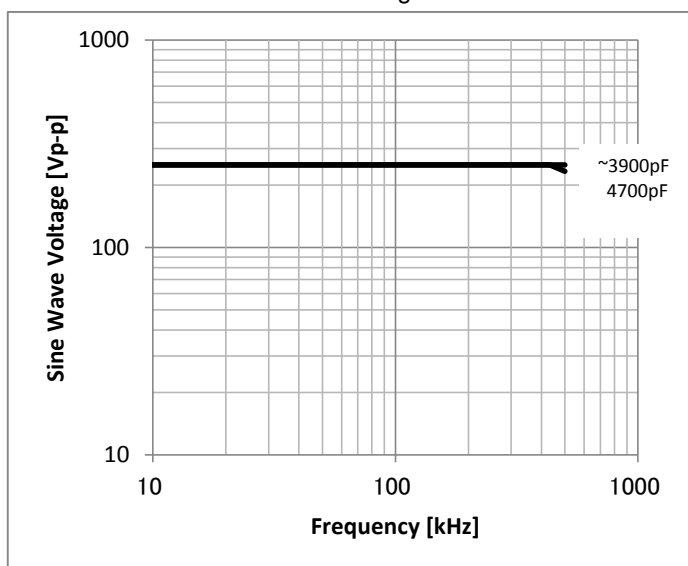
Except for 0805(2012 in mm)/1206(3216 in mm)size C0G Char. Rated Voltage : DC250V
