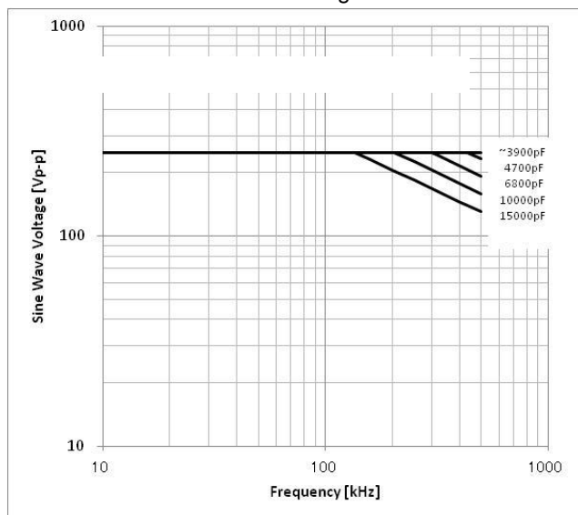
1206(3216 in mm)size C0G Char. Rated Voltage : DC250V
