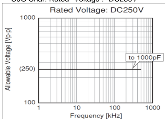
Except for 0805(2012 in mm)/1206(3216 in mm)size C0G Char. Rated Voltage : DC250V
