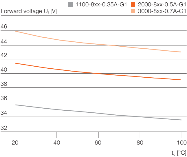
Typical forward voltage as a function of case temperature
