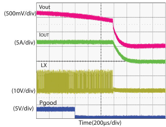
Output Over-Current Response
