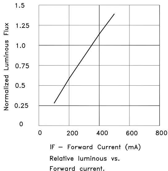
Forward Current Characteristics, TA=25°C
