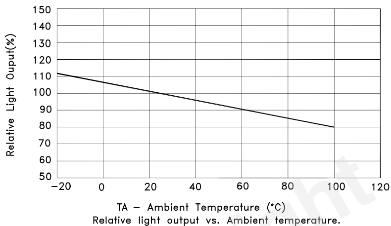
Light Output Characteristics
