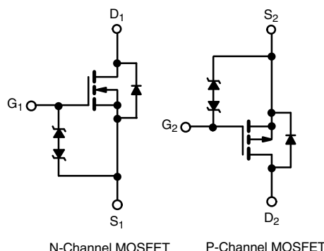
N-Channel MOSFET
