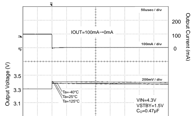
Figure 18. Load Response
