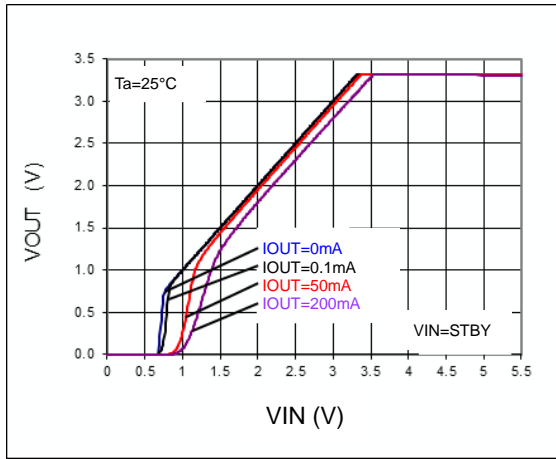
Figure 3. Output Voltage
