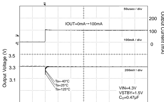
Figure 17. Load Response
