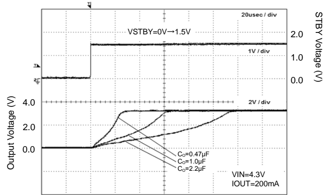
Figure 24. Start Up Time IOU=200mA
