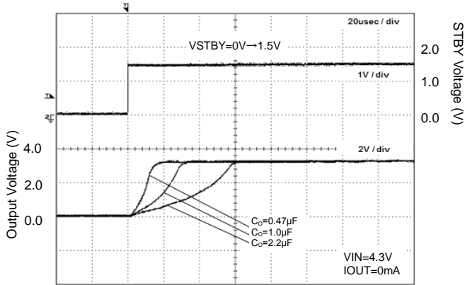
Figure 23. Start Up Time IOU=0mA
