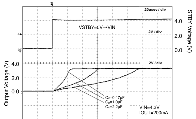
Figure 26. Start Up Time (VIN=STBY) IOU=200mA
