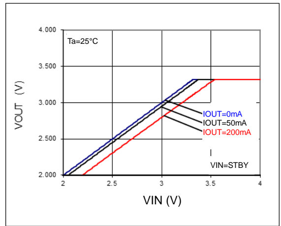
Figure 4. Output Voltage
