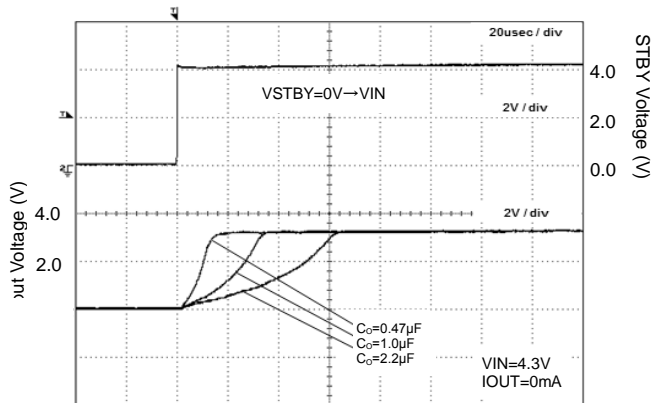
Figure 25. Start Up Time (VIN=STBY) IOU=0mA
