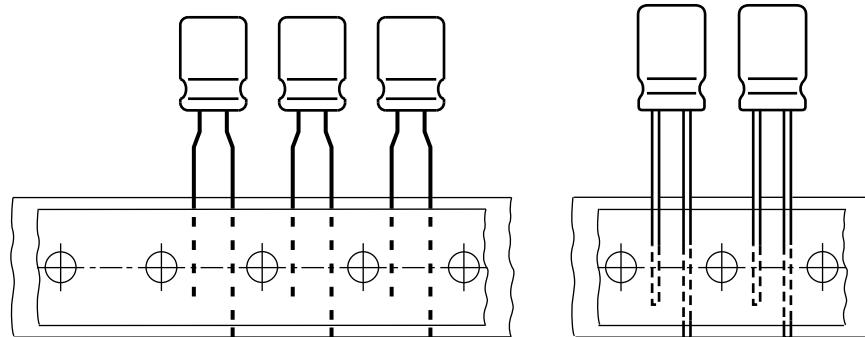
Pitch F = 2.5 \text{ mm} Case \varnothing D = 4 \text{ mm to } 6.3 \text{ mm}
