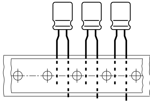
Case \varnothing D = 4 \text{ mm to } 6.3 \text{ mm} ; pitch F = 5 \text{ mm}
