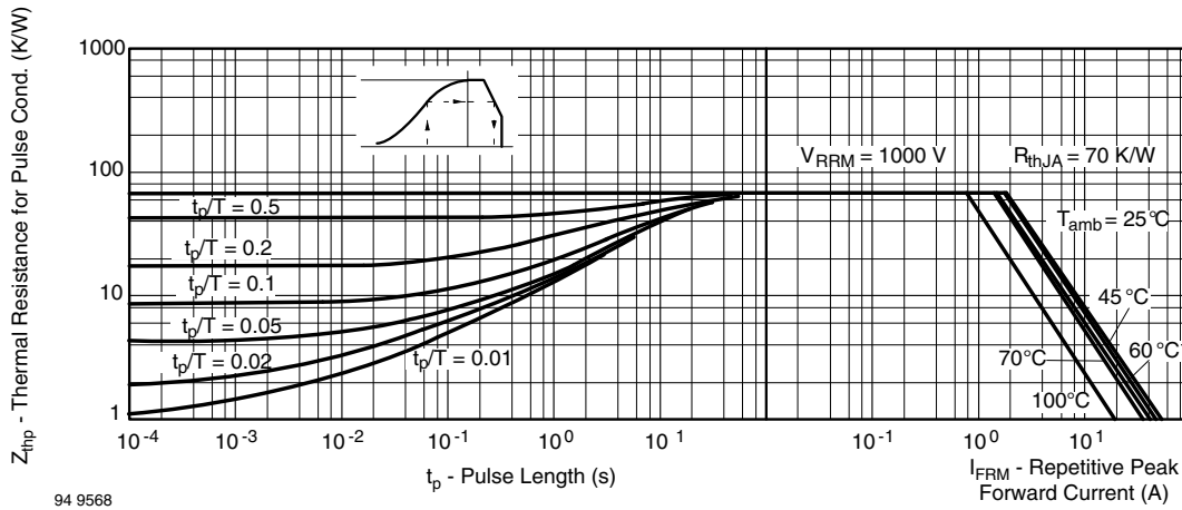
Fig. 7 - Thermal Response
