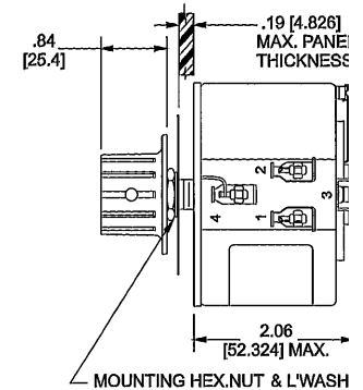
MOUNTING HEX.NUT & L'WASH
