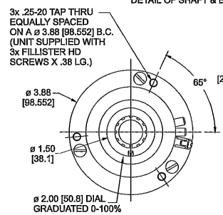
DETAIL OF SHAFT & BUSHING
