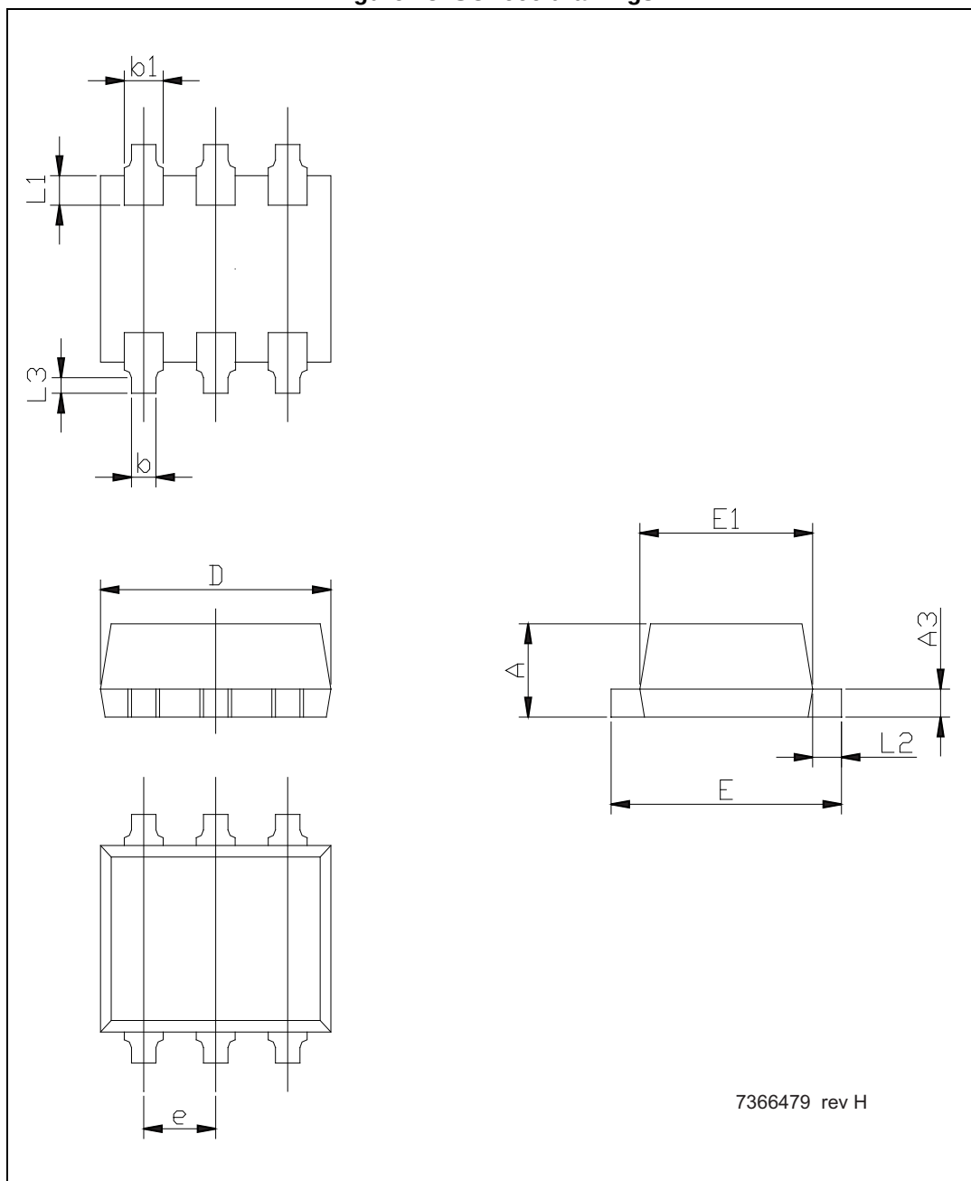
Figure 18. SOT666 drawings
