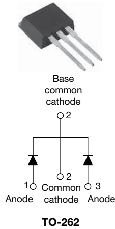
VS-MBR20..CT-1PbF
