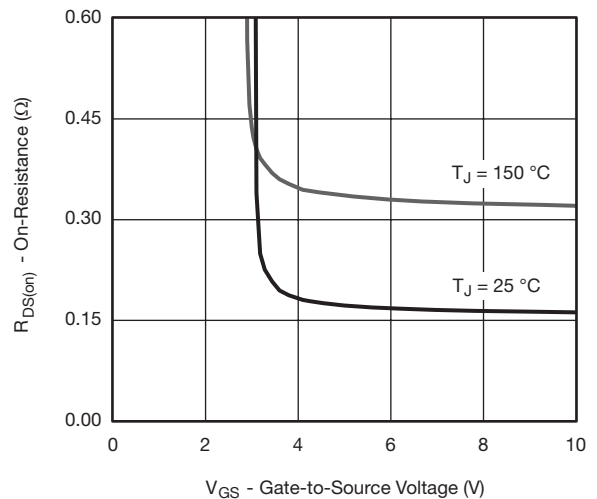
T_J = 150 °C T_J = 25 °C On-Resistance vs. Gate-to-Source Voltage
