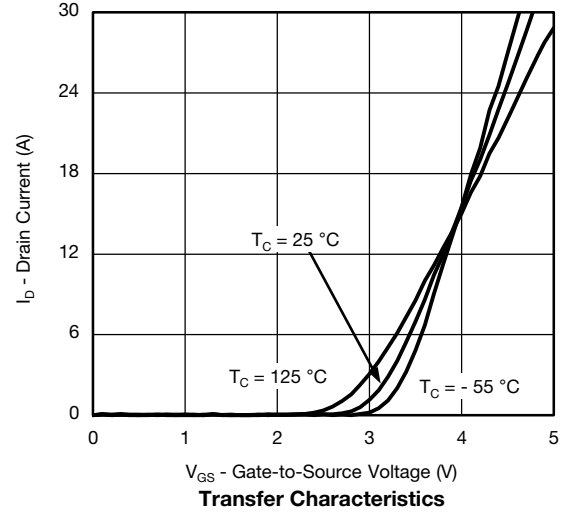
Transfer Characteristics
