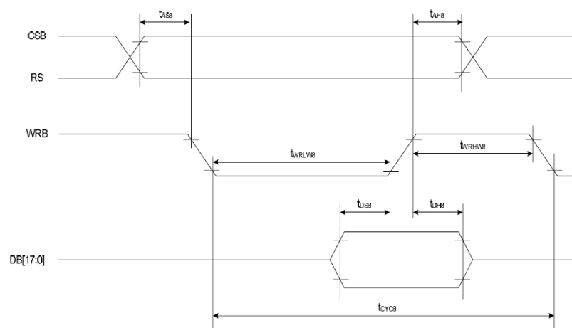
( Write Timing )
