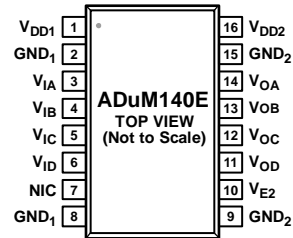
Figure 7. ADuM140E Pin Configuration
