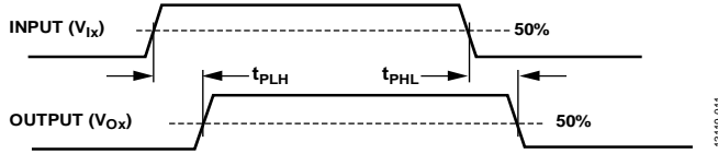
Figure 23. Propagation Delay Parameters
