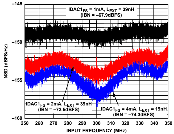
Figure 81. NSD vs. IDAC1_{FS} Setting with Decimate by 16, I/Q Output (IF = 300 MHz, BW = 100 MHz, F_{ADC} = 3.2 \text{ GHz} )
