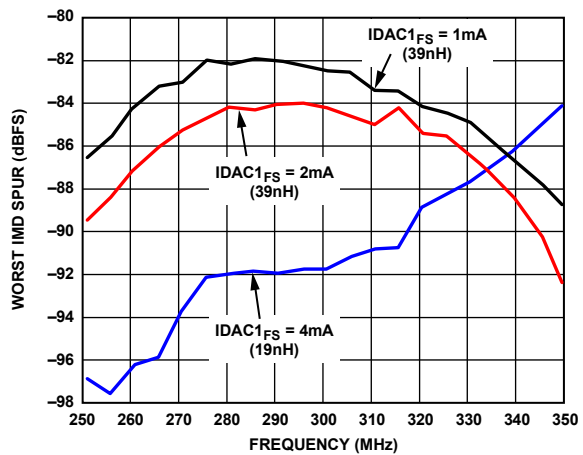
Figure 82. Swept Dual-Tone IMD vs. IDAC1_{FS} Setting with Decimate by 16, I/Q Output, Dual Tones Set to -8 \text{ dBFS} (IF = 300 MHz, BW = 100 MHz, F_{ADC} = 3.2 \text{ GHz} )
