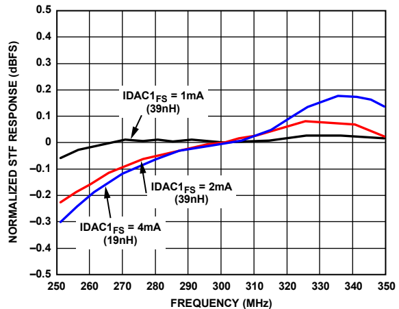
Figure 83. STF vs. IDAC1_{FS} Setting with Decimate by 16, I/Q Output, Dual Tones Set to -8 \text{ dBFS} (IF = 300 MHz, BW = 100 MHz, F_{ADC} = 3.2 \text{ GHz} )
