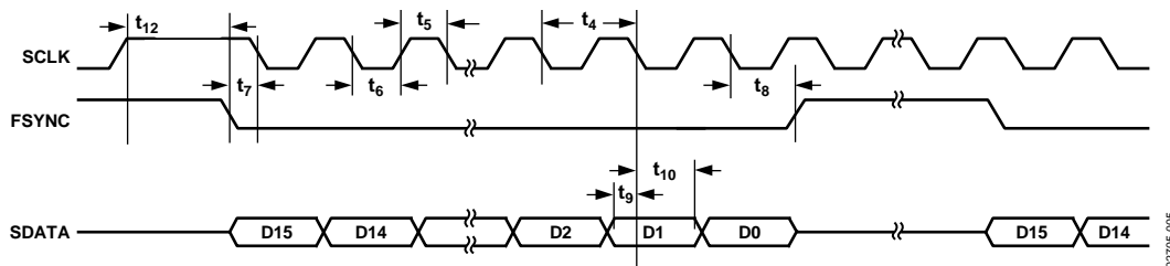
Figure 5. Serial Timing
