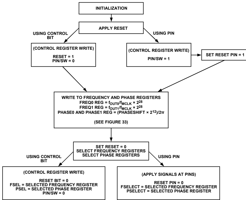
Figure 32. Initialization
