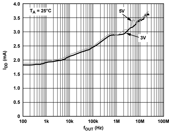
Figure 8. Typical I_{DD} vs. f_{OUT} for f_{MCLK} = 50 MHz
