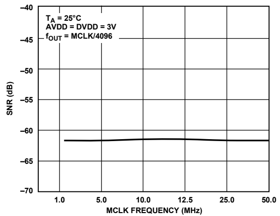
Figure 12. SNR vs. MCLK Frequency
