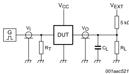
Test data is given in Table 10 . Definitions for test circuit: RL = Load resistance. CL = Load capacitance including jig and probe capacitance. RT = Termination resistance should be equal to the output impedance Zo of the pulse generator. VEXT = External voltage for measuring switching times.
