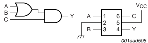
Fig 9. 3-input gate with the Boolean function: Y = (A + B) \times C
