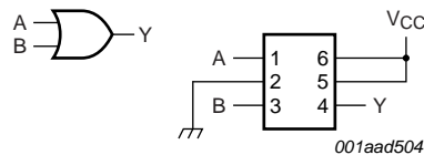
Fig 8. 2-input OR gate
