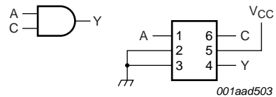
Fig 7. 2-input AND gate
