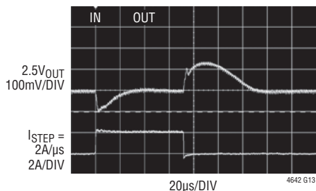
12V IN to 2.5V OUT Transient Response
