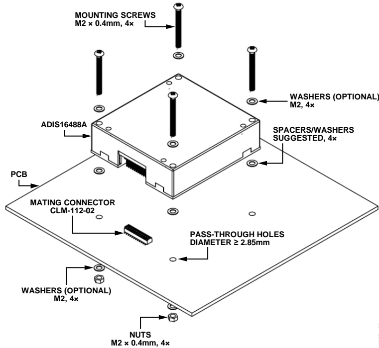
Figure 26. Mounting Example
