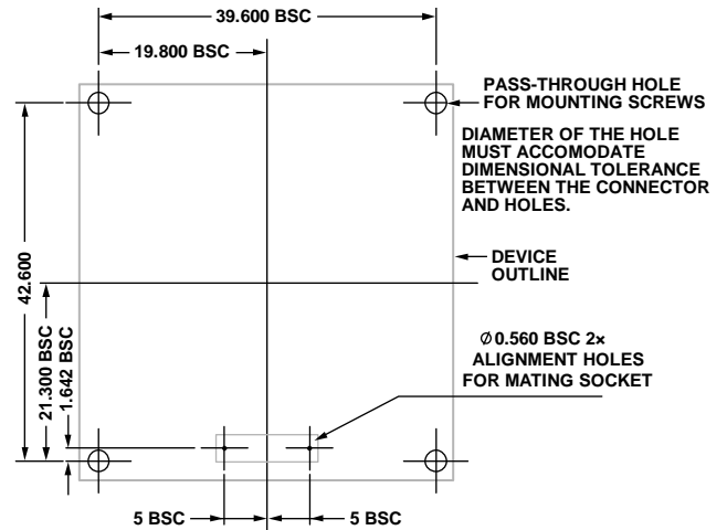
Figure 26. Mounting Example
