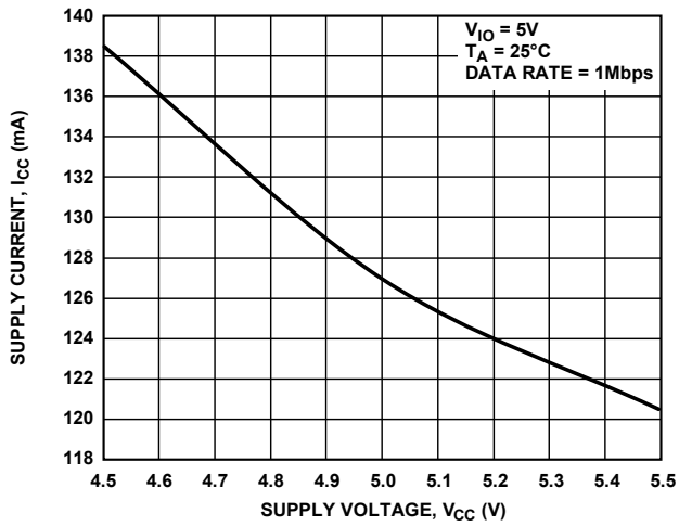
Figure 19. Supply Current, I_{CC} vs. Supply Voltage V_{CC}
