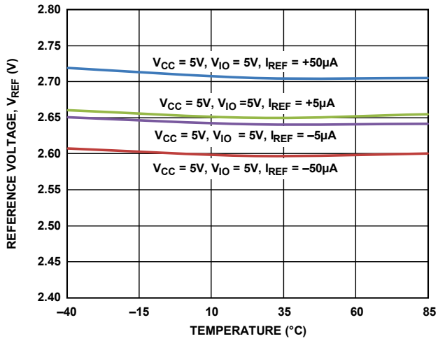
Figure 17. Reference Voltage vs. Temperature
