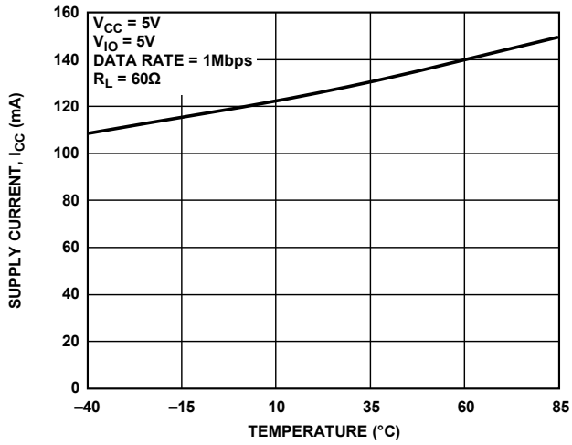
Figure 18. Supply Current I_{CC} vs. Temperature
