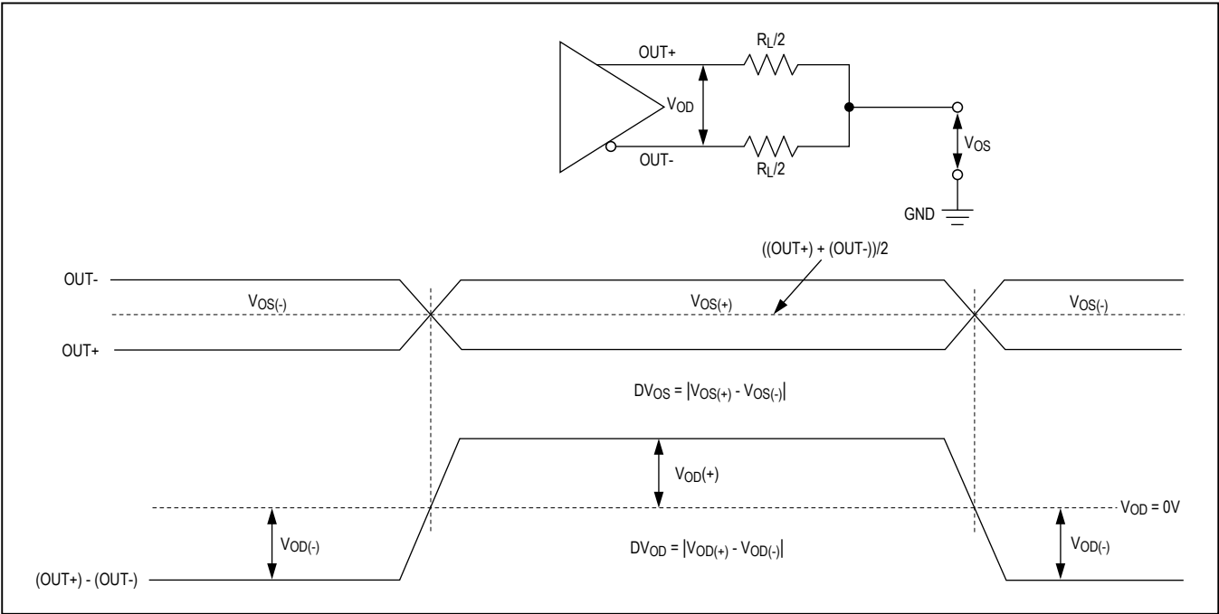
Figure 1. Serial-Output Parameters
