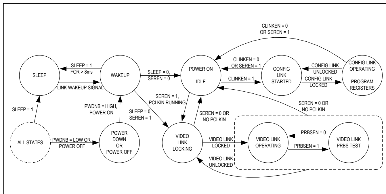
Figure 20. State Diagram
