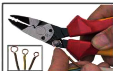
Looping device Ø 4, 5, 6mm
