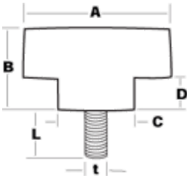
Dimension Chart
