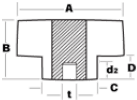
Dimension Chart
