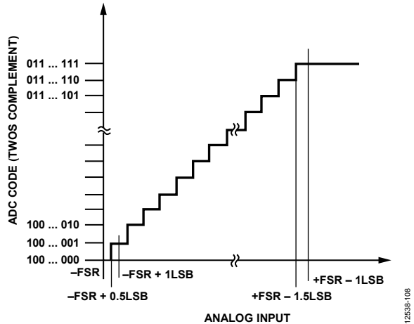
Figure 90. Transfer Function
