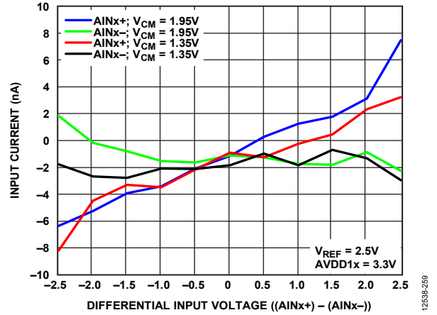
Figure 59. Input Current vs. Differential Input Voltage, Low Power Mode
