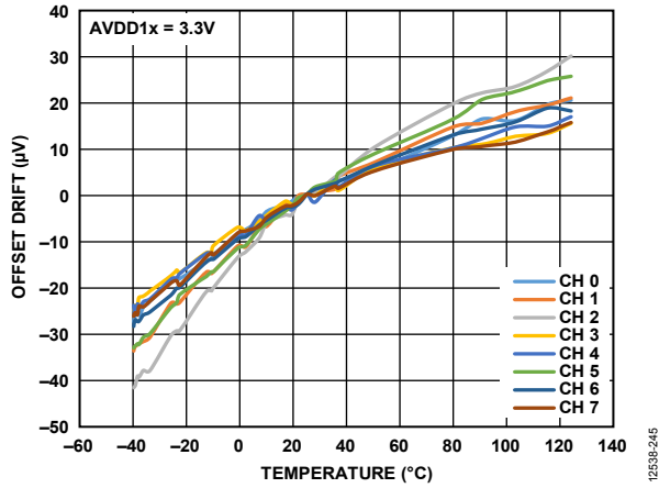
Figure 45. Offset Drift vs. Temperature
