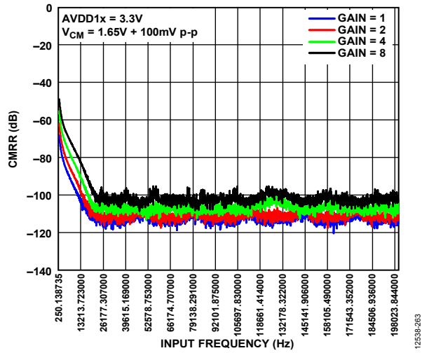
Figure 63. Common-Mode Rejection Ratio (CMRR) vs. Input Frequency at 16 kSPS, High Resolution Mode
