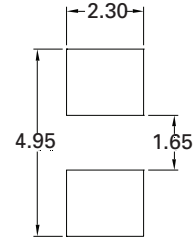
Recommended Pad Layout
