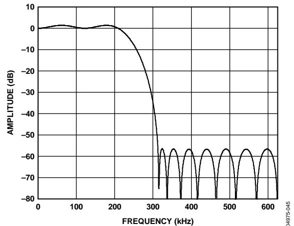
Figure 58. 24-Tap FIR Frequency Response
