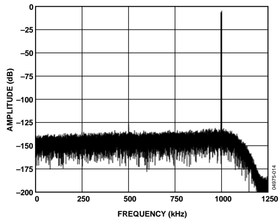
Figure 13. Normal Mode FFT, 1 MHz, -0.5 dB Input Tone, 8× Decimation
