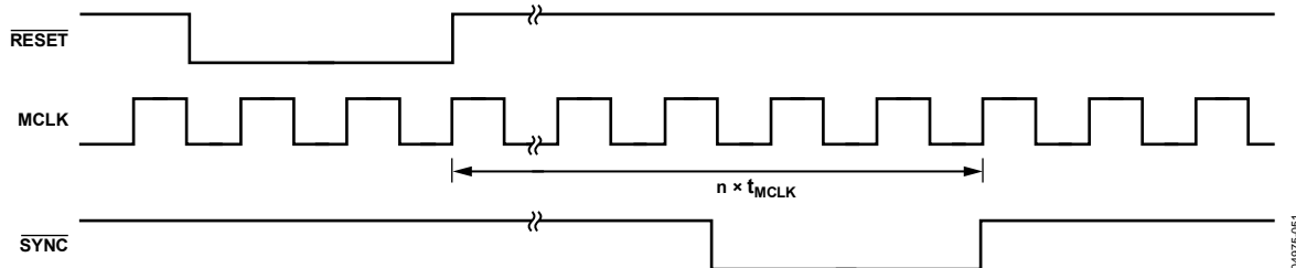
Figure 44. AD7760 Relative Timing Between \overline{\text{RESET}} and \overline{\text{SYNC}} in Modulator Output Mode \overline{\text{CDIV}} = 0
