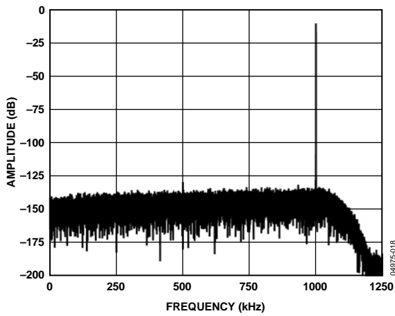
Figure 17. Normal Mode FFT, 1 MHz, -6 dB Input Tone, 8x Decimation
