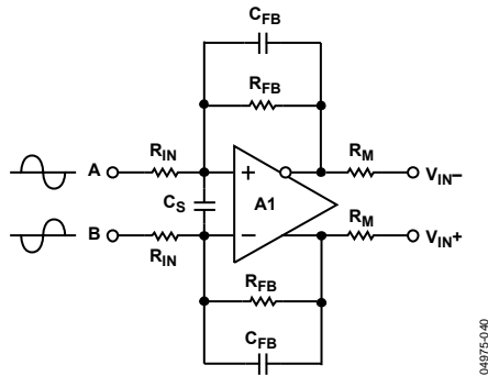
Figure 50. Differential Amplifier Configuration
