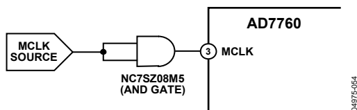
Figure 47. Buffering the MCLK Signal Using the NC7SZ08M5 AND Gate
