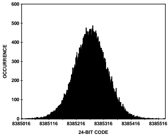
Figure 30. Normal Mode, 24-Bit Histogram, 8x Decimation
