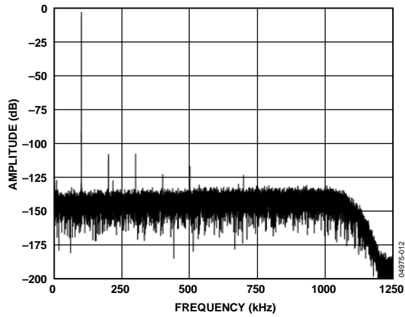
Figure 11. Normal Mode FFT, 100 kHz, -0.5 dB Input Tone, 8× Decimation
