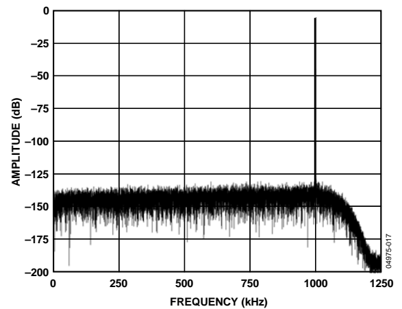
Figure 16. Low Power FFT, 1 MHz, -0.5 dB Input Tone, 8× Decimation
