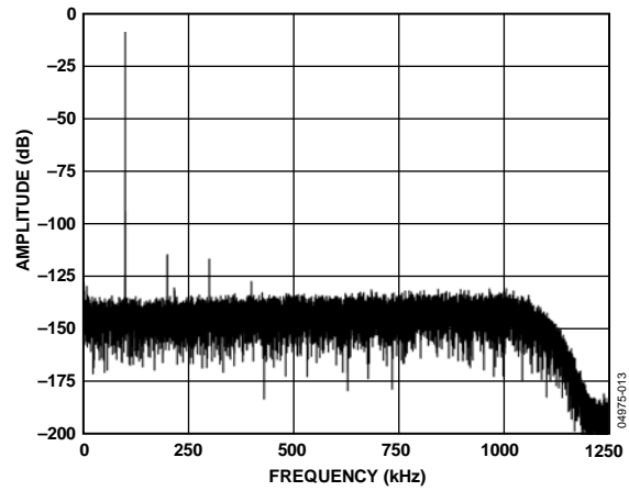
Figure 12. Normal Mode FFT, 100 kHz, -6 dB Input Tone, 8× Decimation
