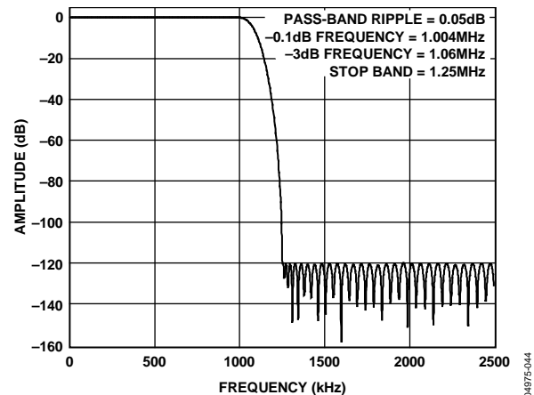
Figure 57. Default Filter Frequency Response (2.5 MHz ODR)
