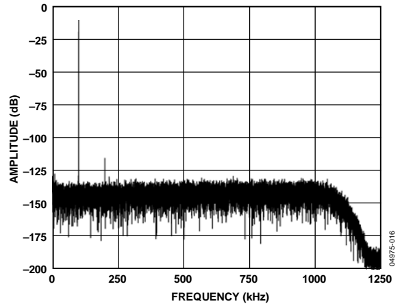
Figure 15. Low Power FFT, 100 kHz, -6 dB Input Tone, 8× Decimation
