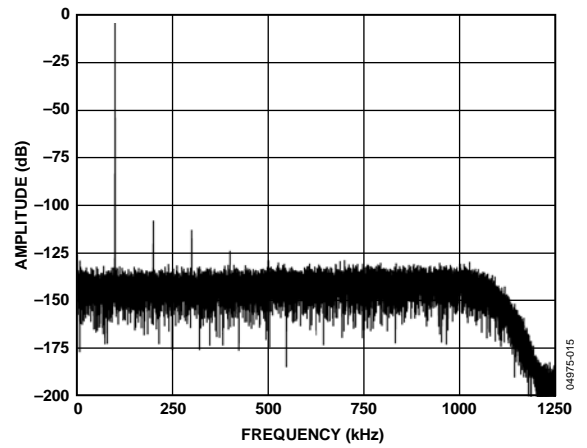
Figure 14. Low Power FFT, 100 kHz, -0.5 dB Input Tone, 8× Decimation
