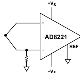
THERMOCOUPLE
