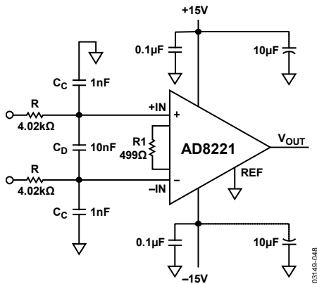
Figure 49. RF Interference Suppression
