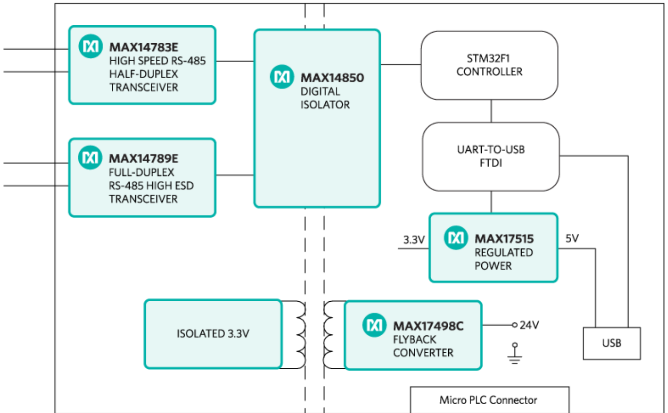
Figure 1, The MAXREFDES62# reference design block diagram.
