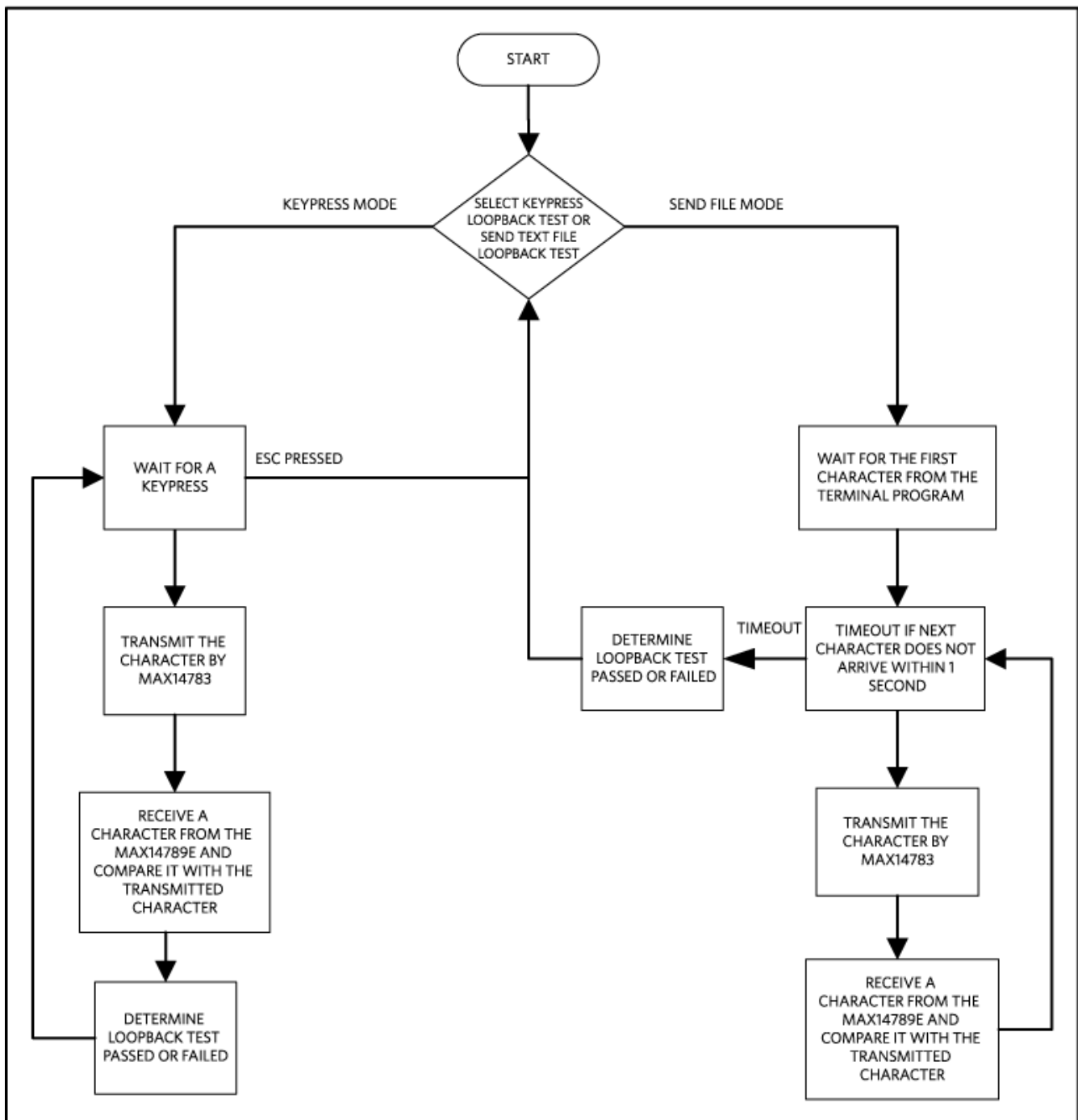
Figure 2, The MAXREFDES62# firmware flowchart
