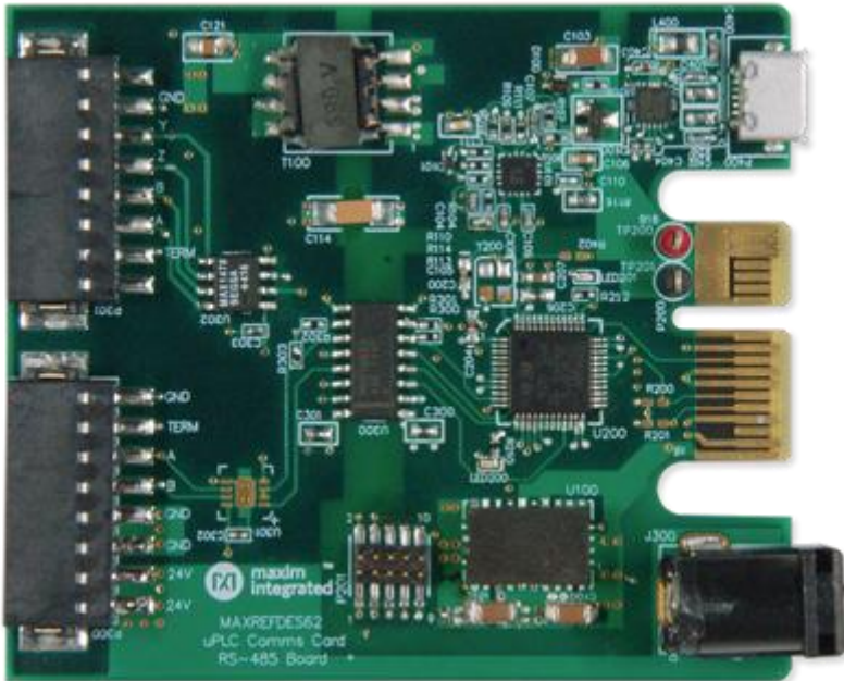
MAXREFDES39# System Board
