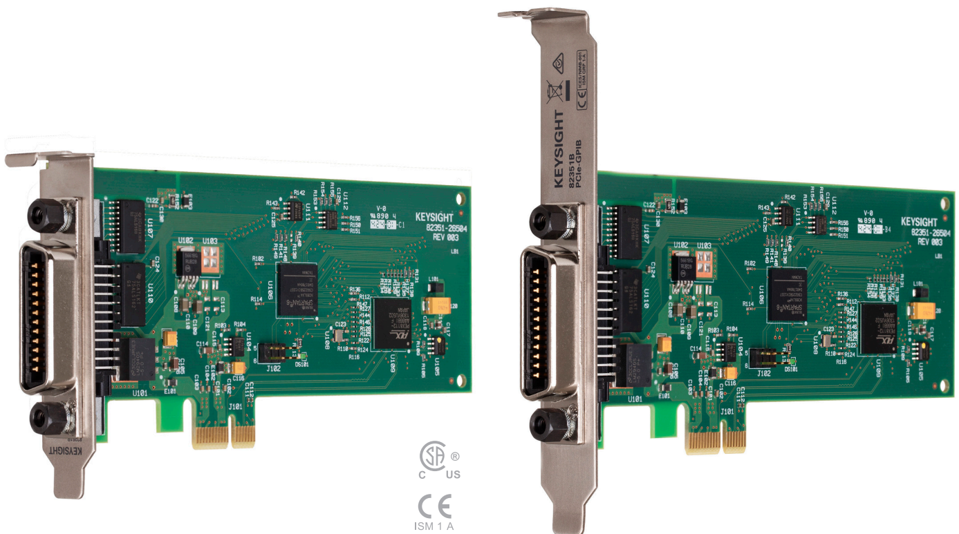
82351B with standard (right) and low-profile (left) brackets
