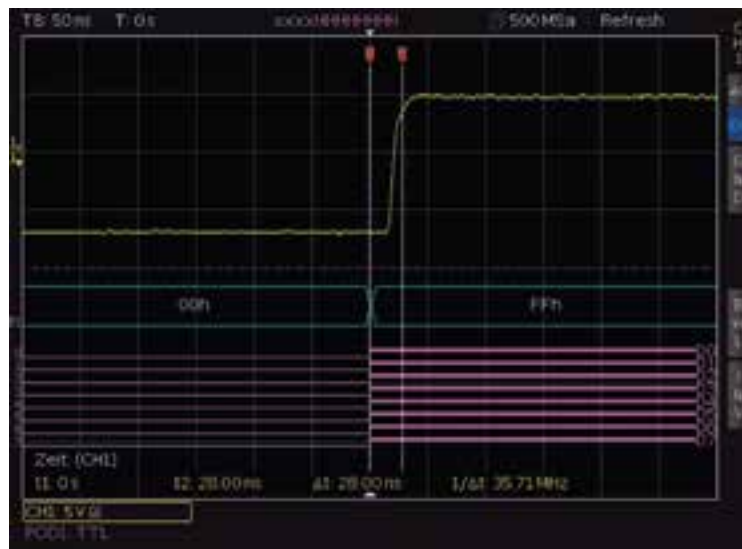
Eight-bit DAC signal change.
