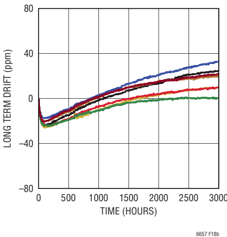
Figure 18b. Long-Term Drift MS8 Burn-In 150^\circ\text{C}/24\text{H}
