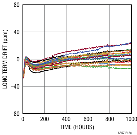
Figure 18a. Long-Term Drift MS8
