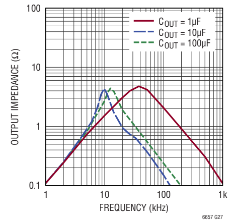
5V Output Impedance vs Frequency
