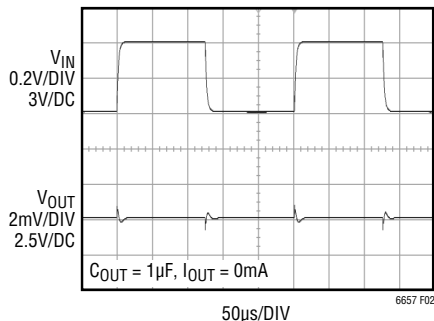
Figure 2. Line Transient Response with V_{IN} = 0.4V_{p-p}
