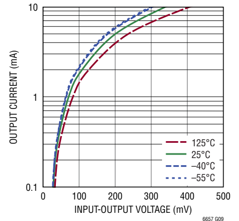
2.5V Minimum V_{IN} to V_{OUT} Differential (Sourcing)
