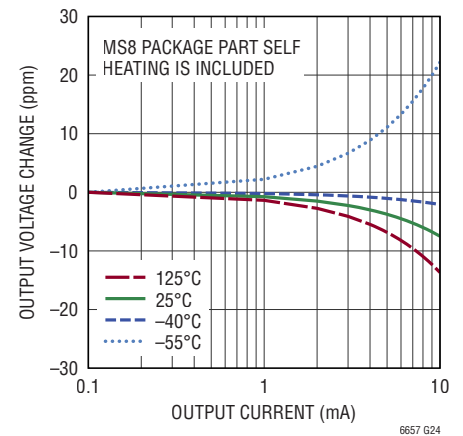
5V Load Regulation (Sinking)
