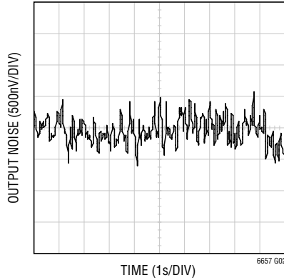
2.5V Low Frequency 0.1Hz to 10Hz Noise
