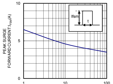
I_{FSM}-t CHARACTERISTICS
