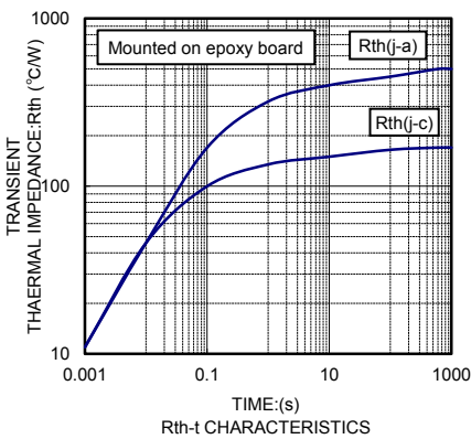
R_{th}-t CHARACTERISTICS
