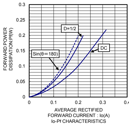
I_o-P_R CHARACTERISTICS
