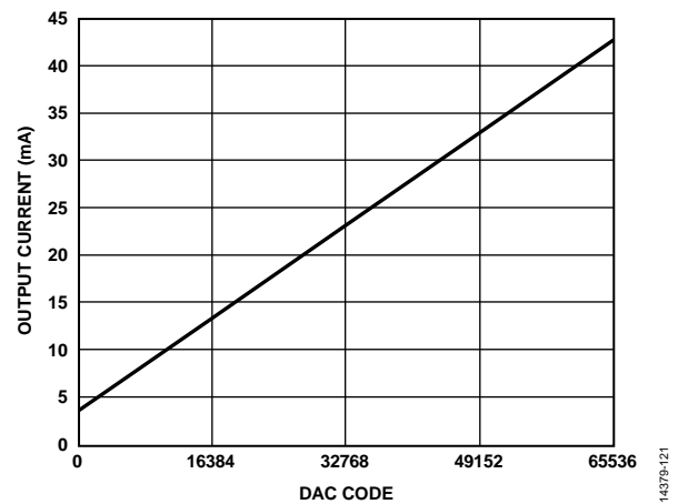
Figure 189. Gain Curve for ANA_FULL_SCALE_CURRENT[9:0] = 1023, DAC Offset = 3.8 mA
