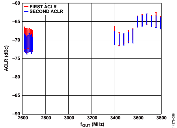
Figure 109. Four-Carrier, W-CDMA ACLR vs. f_{OUT} (First ACLR, Second ACLR)
