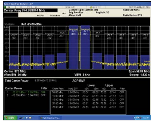
Figure 26. Two-Carrier W-CDMA at 875 MHz
