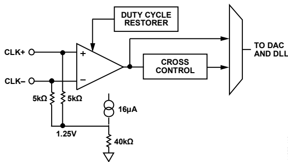
Figure 184. Clock Input
