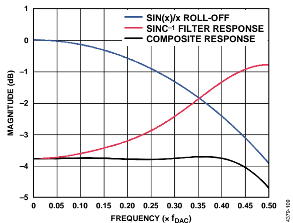
Figure 172. Responses of \sin(x)/x Roll-Off, the \text{Sinc}^{-1} Filter, and the Composite of the Two
