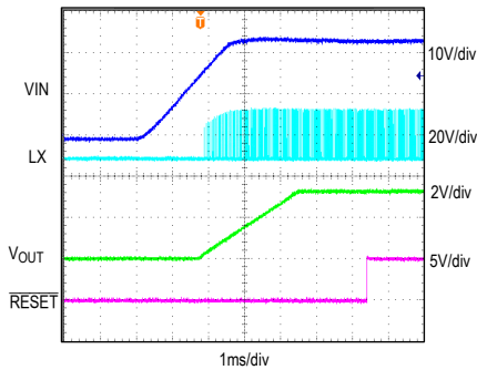
STARTUP THROUGH INPUT SUPPLY VIN = 24V, VOUT = 3.3V, IOUT = 1.7A, MODE = SGND toc33
