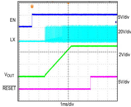
STARTUP THROUGH ENABLE VIN = 24V, VOUT = 5V, IOUT = 0A, MODE = SGND toc35
