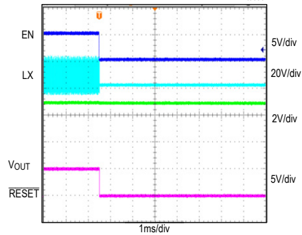
SHUTDOWN THROUGH ENABLE VIN = 24V, VOUT = 5V, IOUT = 0A, MODE = SGND toc36
