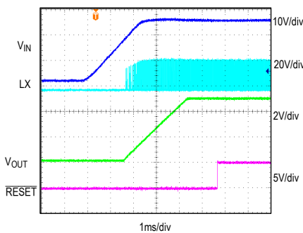
STARTUP THROUGH INPUT SUPPLY VIN = 24V, VOUT = 5V, IOUT = 1.7A, MODE = SGND toc37
