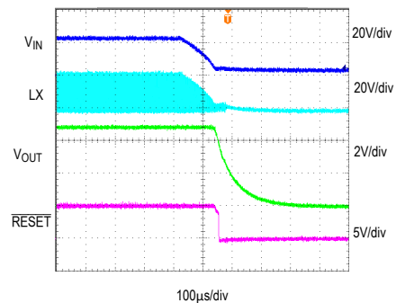
SHUTDOWN THROUGH INPUT SUPPLY VIN = 24V, VOUT = 5V, IOUT = 1.7A, MODE = SGND toc38
