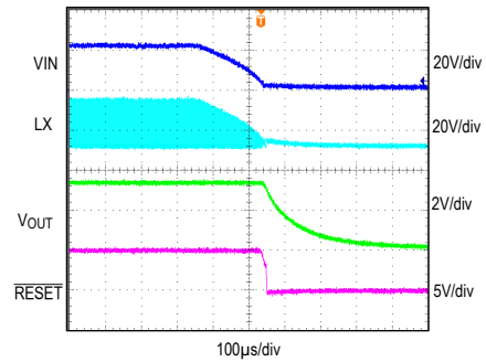
SHUTDOWN THROUGH INPUT SUPPLY VIN = 24V, VOUT = 3.3V, IOUT = 1.7A, MODE = SGND toc34
