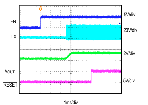
STARTUP WITH 2.5V PREBIAS
