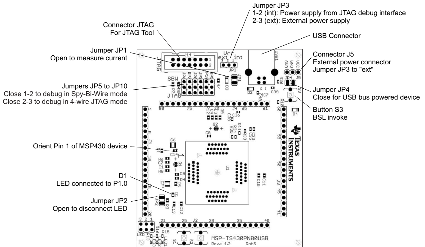
Figure B-56. MSP-TS430PN80USB Target Socket Module, PCB
