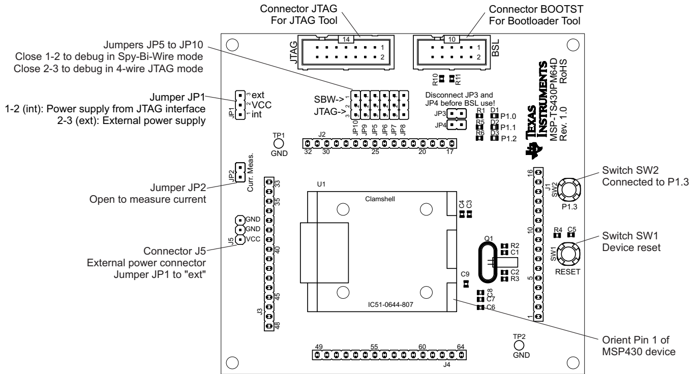
Figure B-42. MSP-TS430PM64D Target Socket Module, PCB
