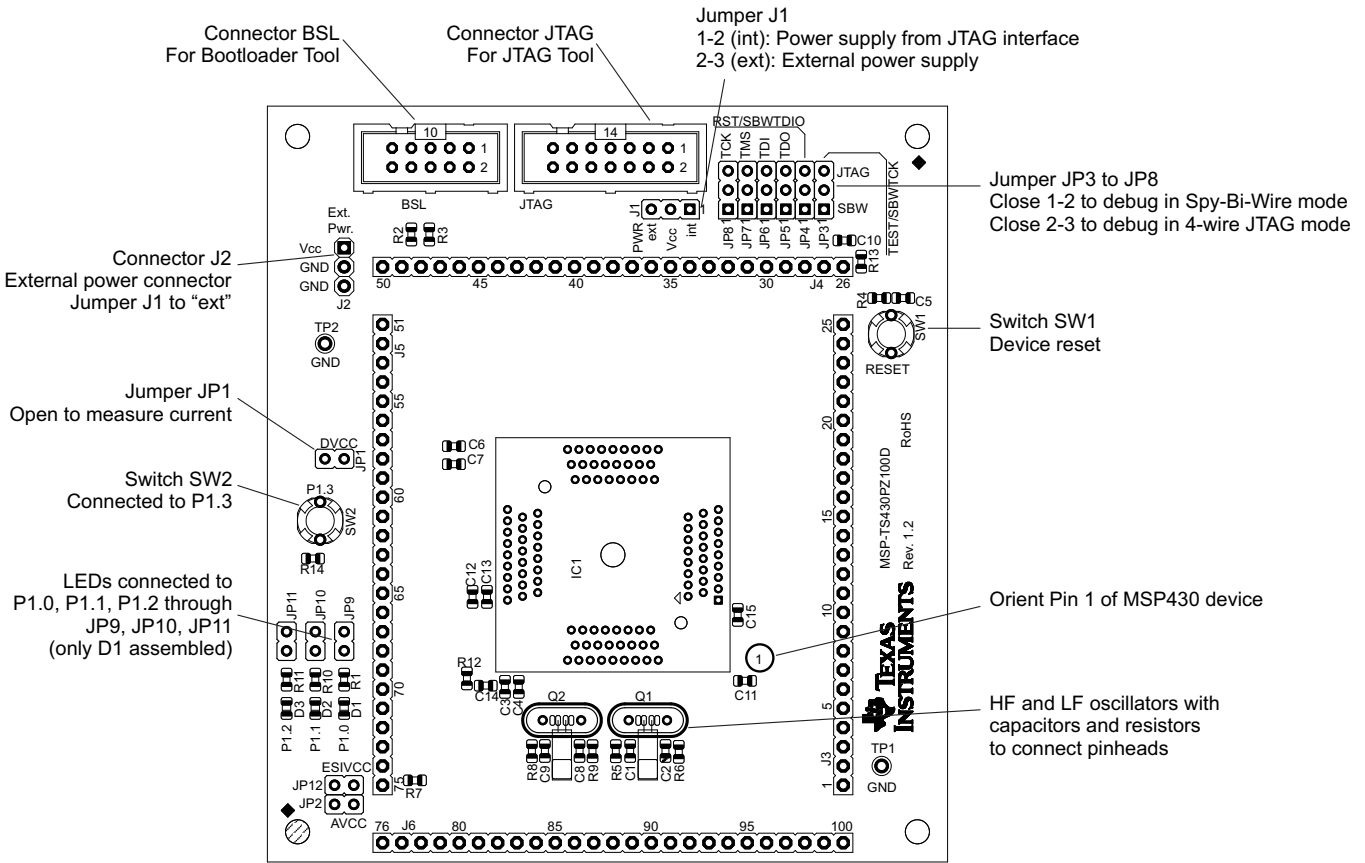
Figure B-66. MSP-TS430PZ100D Target Socket Module, PCB
