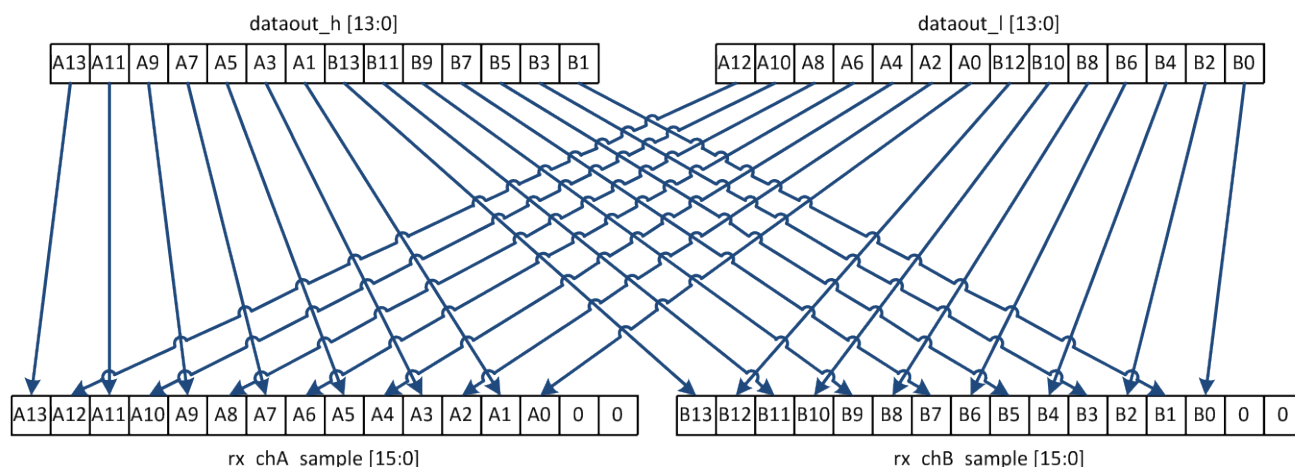
Figure 7. Arrangement and Reordering of ADC Bits out of the ALTDDIO_IN Function
