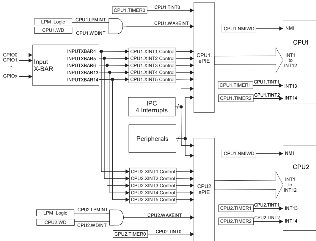
Figure 5-14. External and ePIE Interrupt Sources
