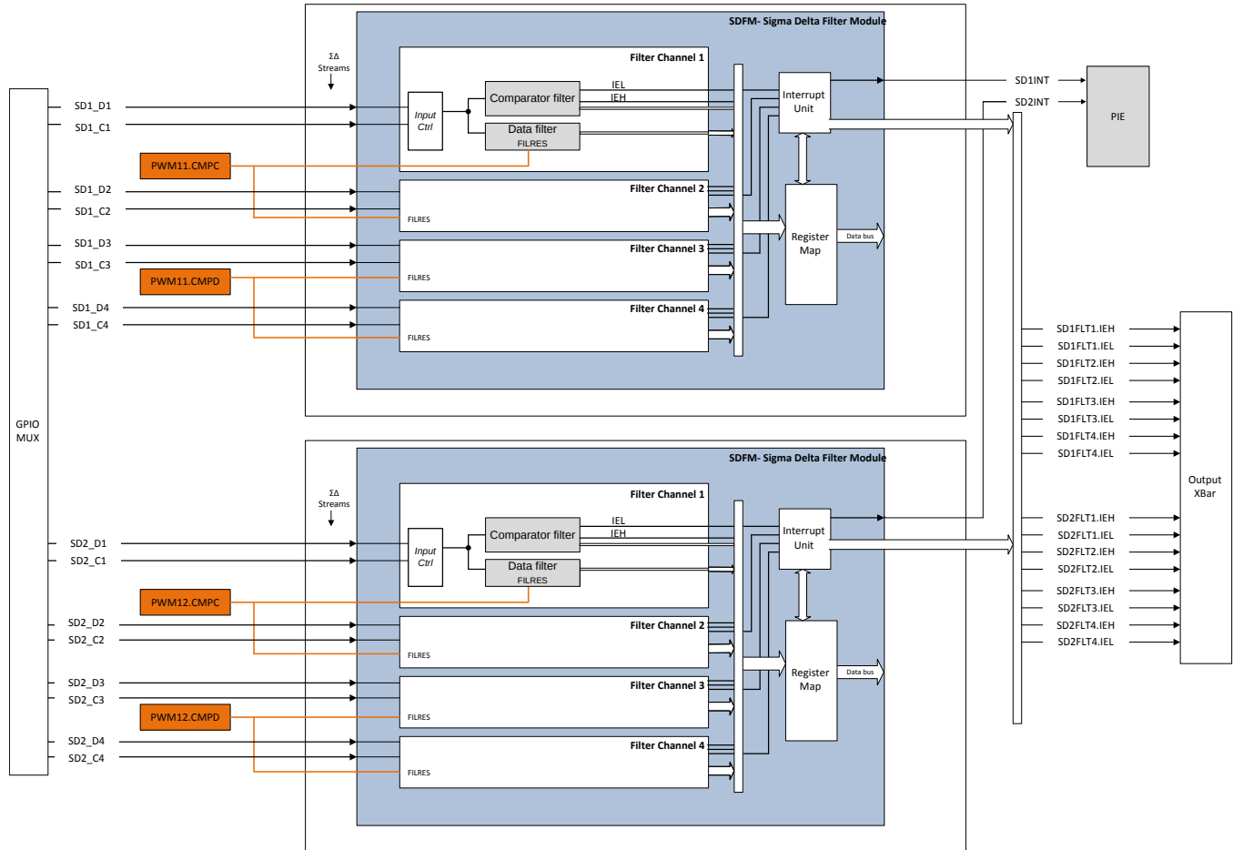
Figure 5-52. SDFM Block Diagram
