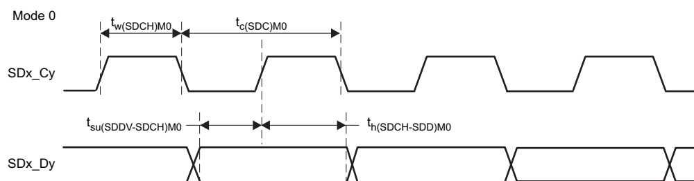
Figure 5-53. SDFM Timing Diagram – Mode 0
