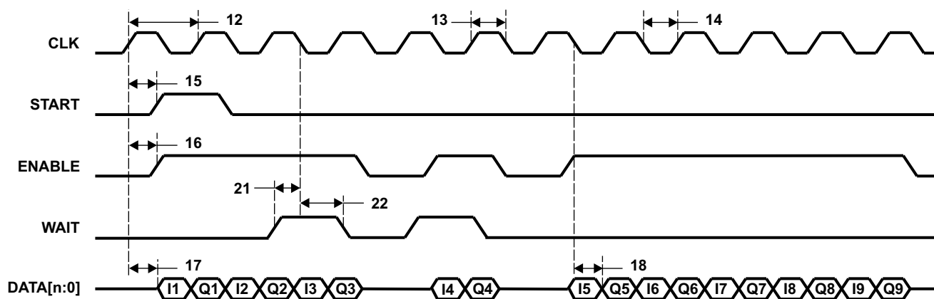
Figure 5-81. uPP Double Data Rate (DDR) Transmit Timing
