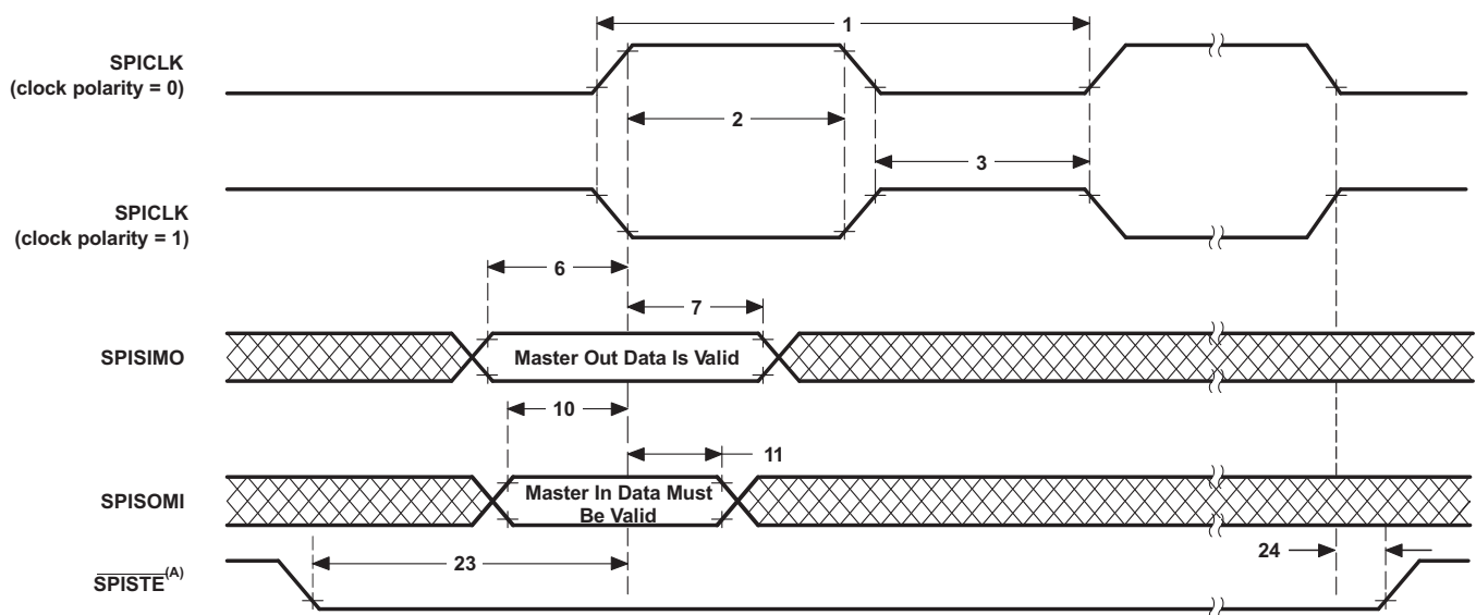
Figure 5-72. High-Speed SPI Master Mode External Timing (Clock Phase = 1)
