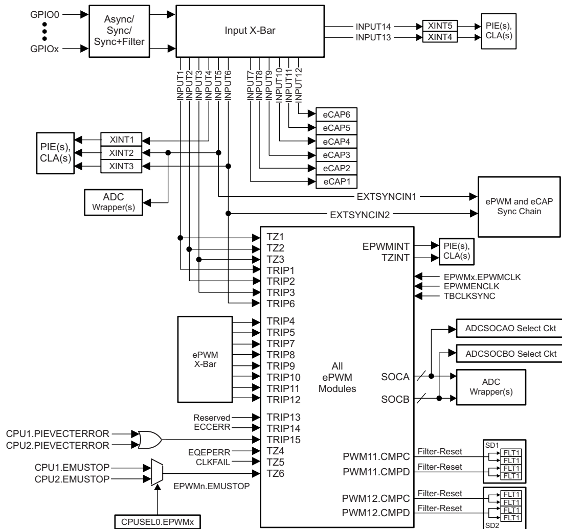
Figure 5-47. ePWM Trip Input Connectivity
