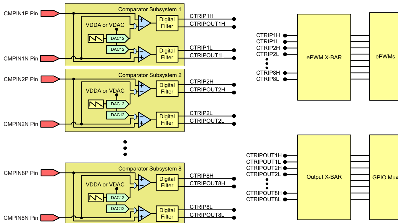
Figure 5-34. CMPSS Connectivity (337-Ball ZWT and 176-Pin PTP)
