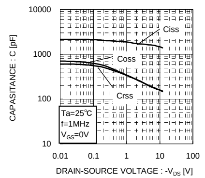
Fig.12 Typical Capacitance vs. Drain-Source Voltage
