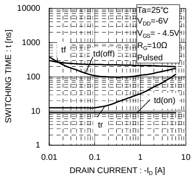
Fig.13 Switching Characteristics
