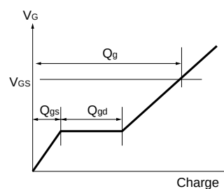
Fig.2-2 Gate Charge Waveforms
