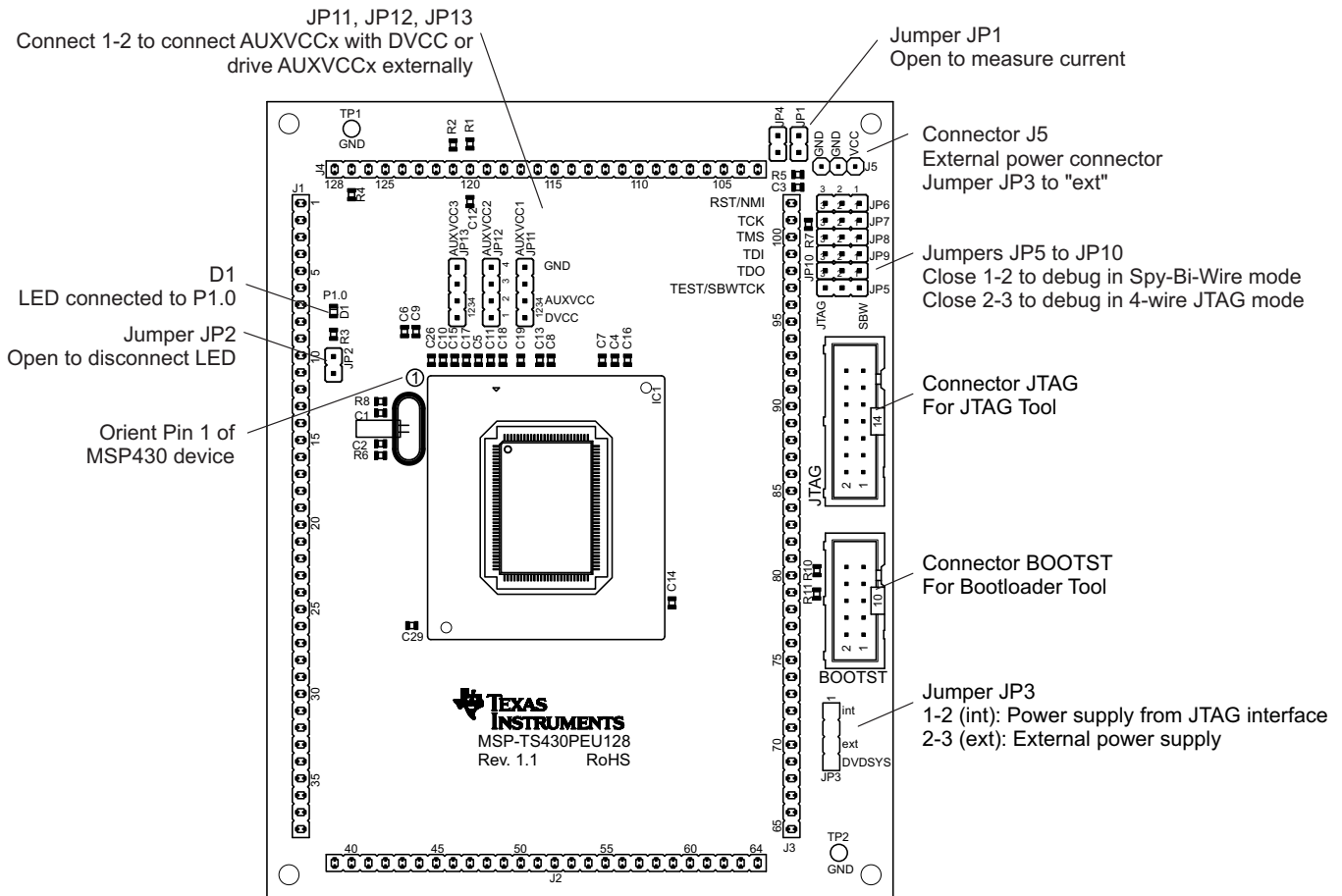
Figure B-75. MSP-TS430PEU128 Target Socket Module, PCB
