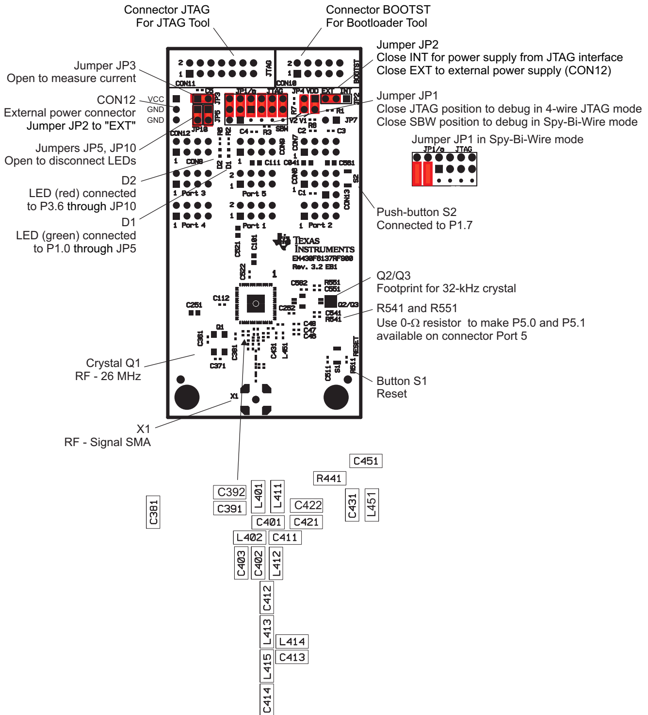
Figure B-79. EM430F6137RF900 Target Board, PCB
