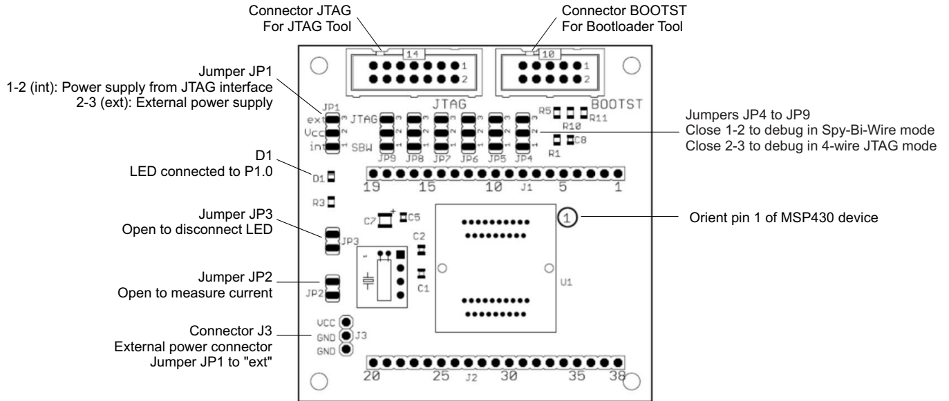
Figure B-25. MSP-TS430DA38 Target Socket Module, PCB
