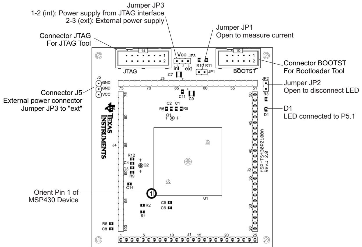
Figure B-61. MSP-TS430PZ100A Target Socket Module, PCB
