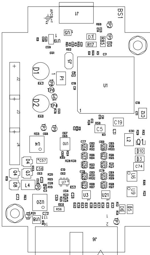
Figure B-89. MSP-FET USB Debugger, PCB (Top)
