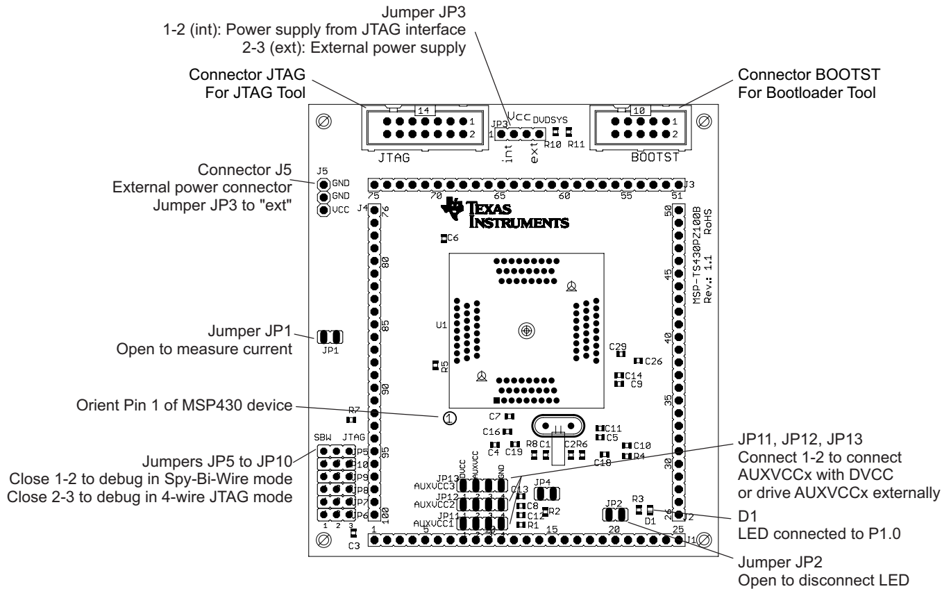
Figure B-63. MSP-TS430PZ100B Target Socket Module, PCB
