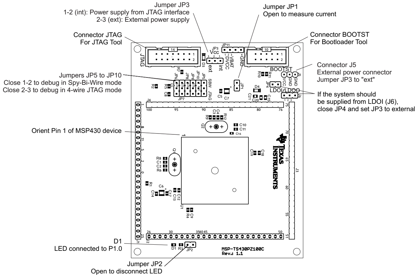
Figure B-65. MSP-TS430PZ100C Target Socket Module, PCB
