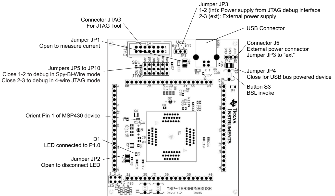
Figure B-57. MSP-TS430PN80USB Target Socket Module, PCB
