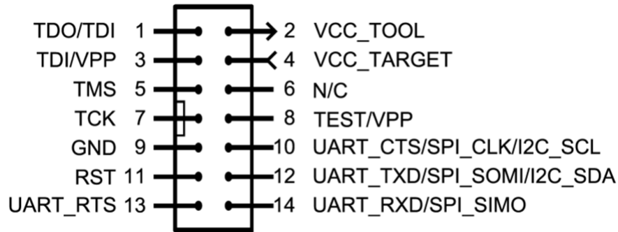
Figure B-91. JTAG Connector Pinout
