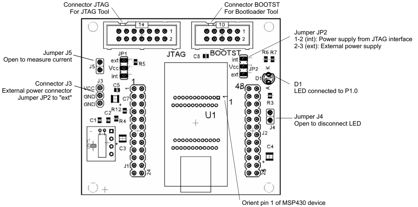
Figure B-33. MSP-TS430DL48 Target Socket Module, PCB
