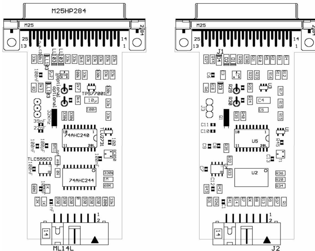
Figure B-99. MSP-FET430PIF FET Interface Module, PCB
