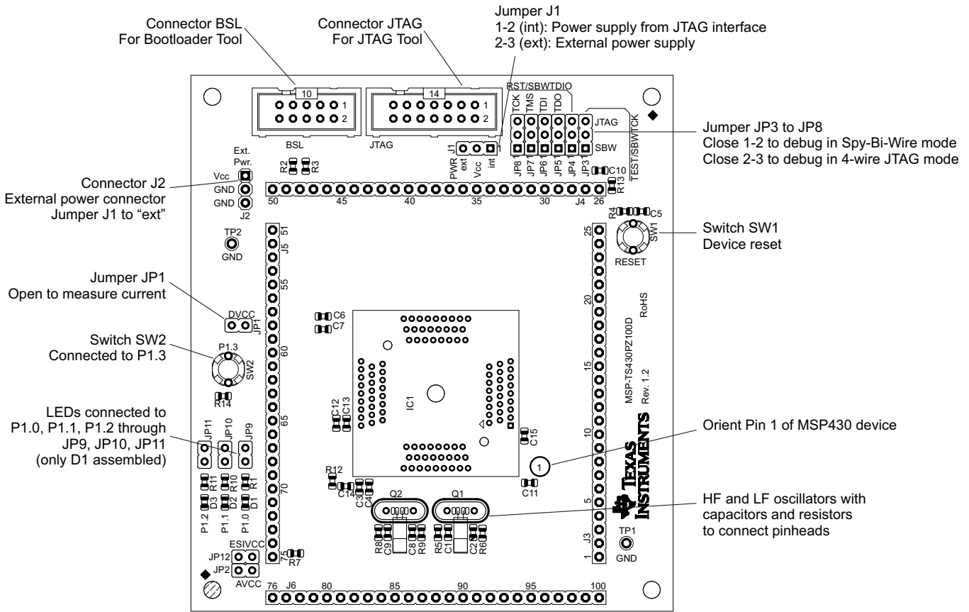
Figure B-67. MSP-TS430PZ100D Target Socket Module, PCB
