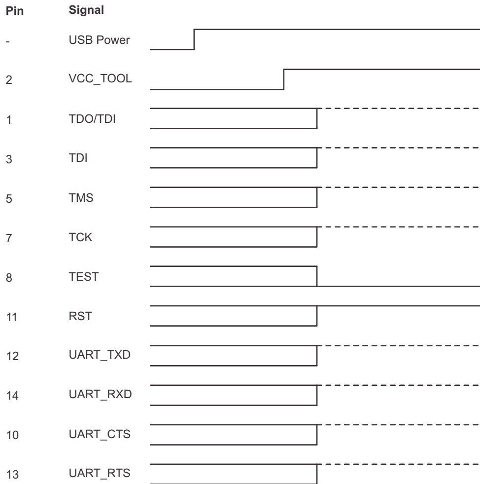
Figure B-92. Pin States After Power-Up
