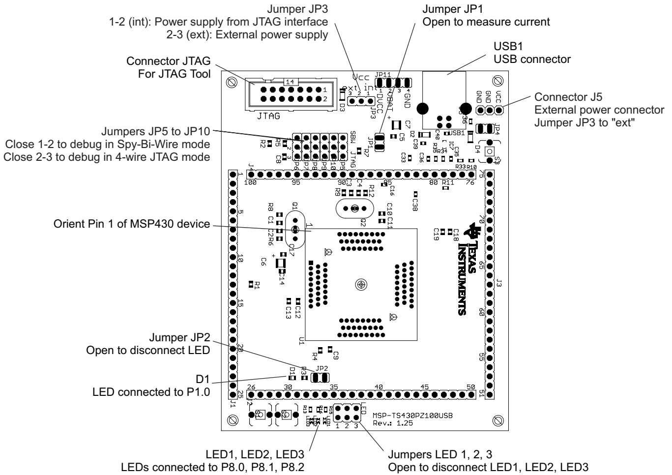
Figure B-71. MSP-TS430PZ100USB Target Socket Module, PCB
