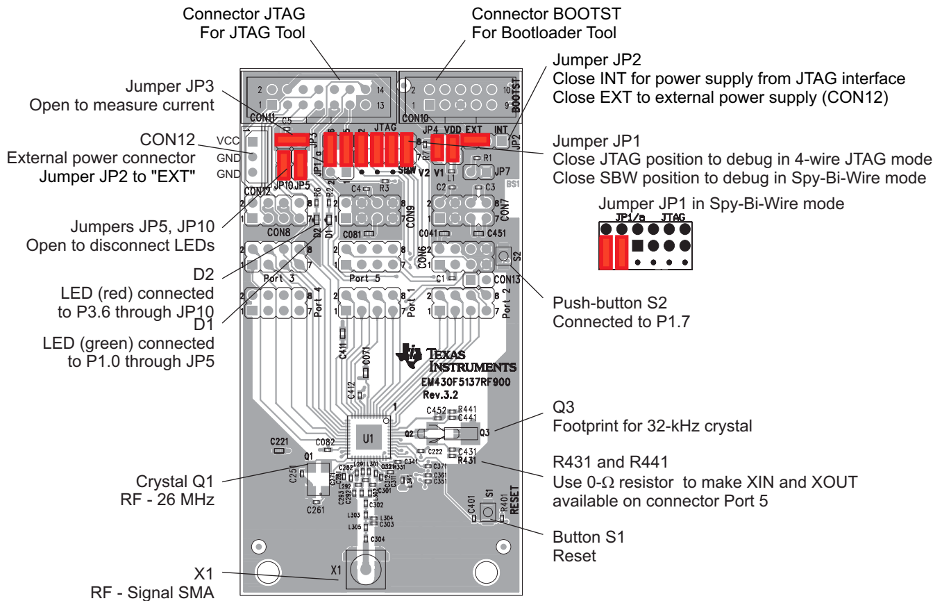
Figure B-77. EM430F5137RF900 Target board, PCB
