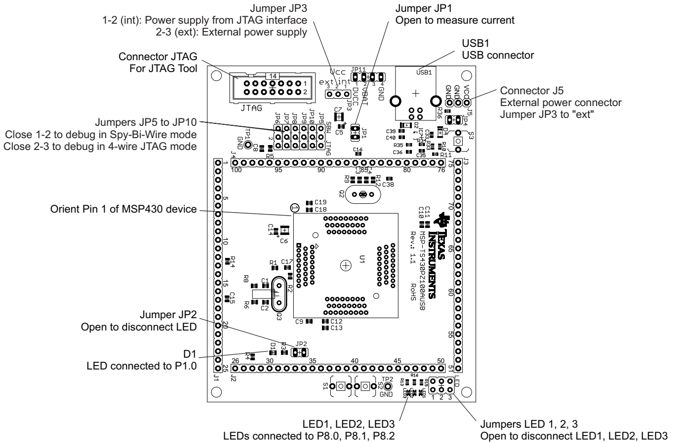
Figure B-73. MSP-TS430PZ100AUSB Target Socket Module, PCB
