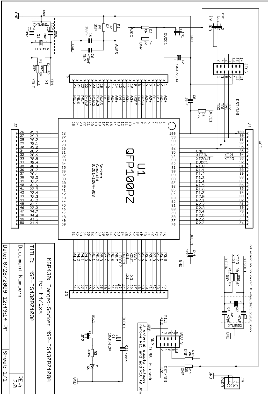
Figure B-60. MSP-TS430PZ100A Target Socket Module, Schematic
