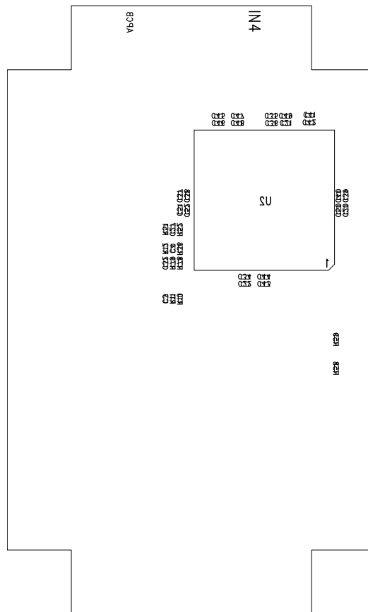
Figure B-90. MSP-FET USB Debugger, PCB (Bottom)
