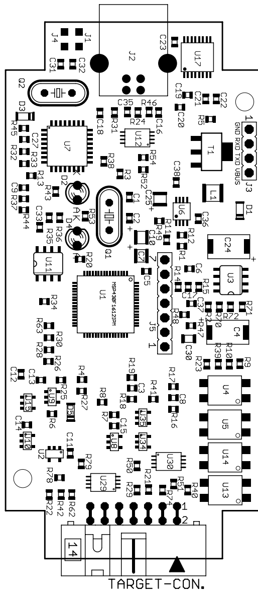
Figure B-97. MSP-FET430UIF USB Interface, PCB
