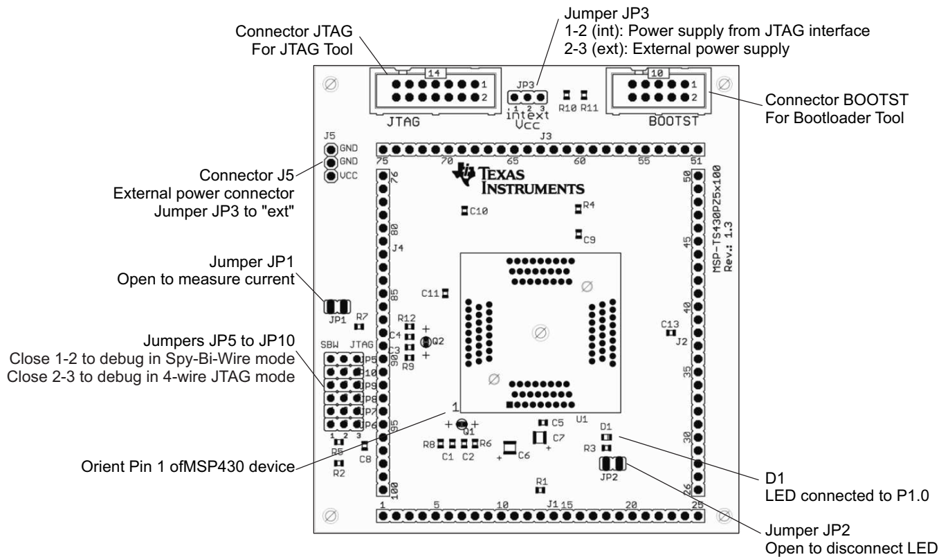
Figure B-69. MSP-TS430PZ5x100 Target Socket Module, PCB
