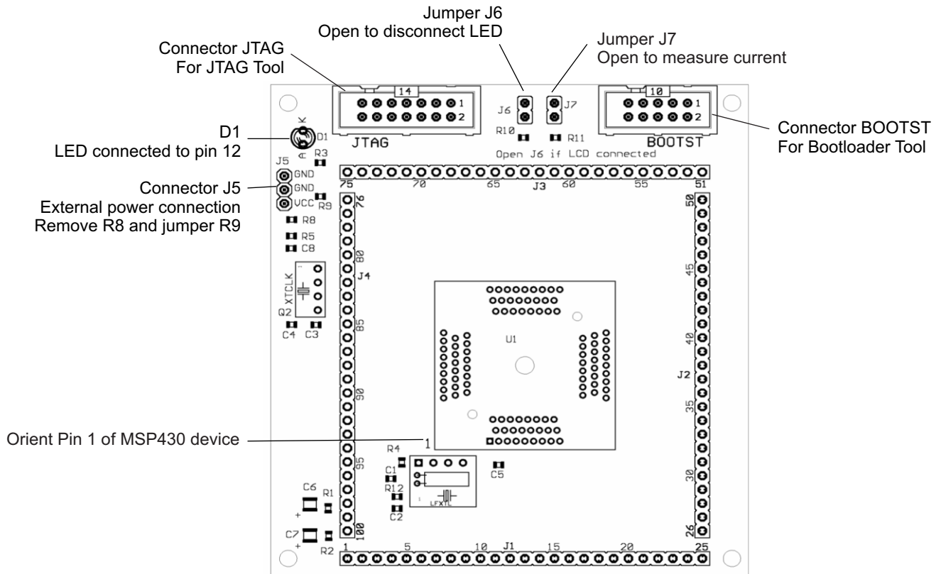
Figure B-59. MSP-TS430PZ100 Target Socket Module, PCB
