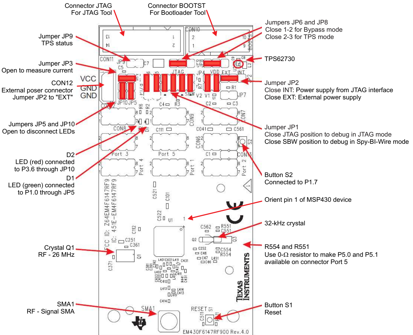
Figure B-81. EM430F6147RF900 Target Board, PCB
