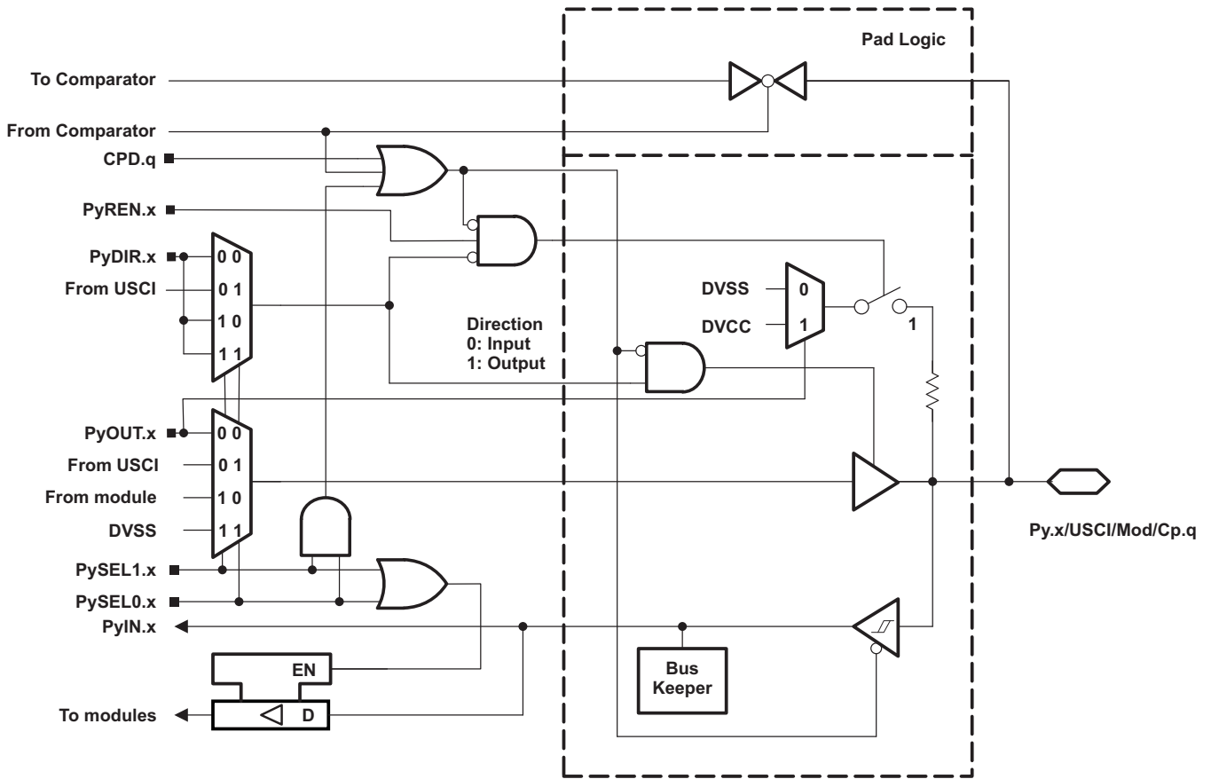
Figure 6-23. Py.x/USCI/Mod/Cp.q Pin Schematic
