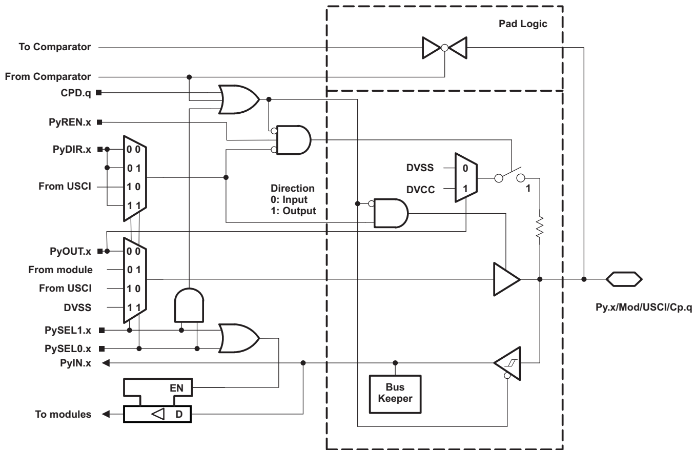
Figure 6-22. Py.x/Mod/USCI/Cp.q Pin Schematic
