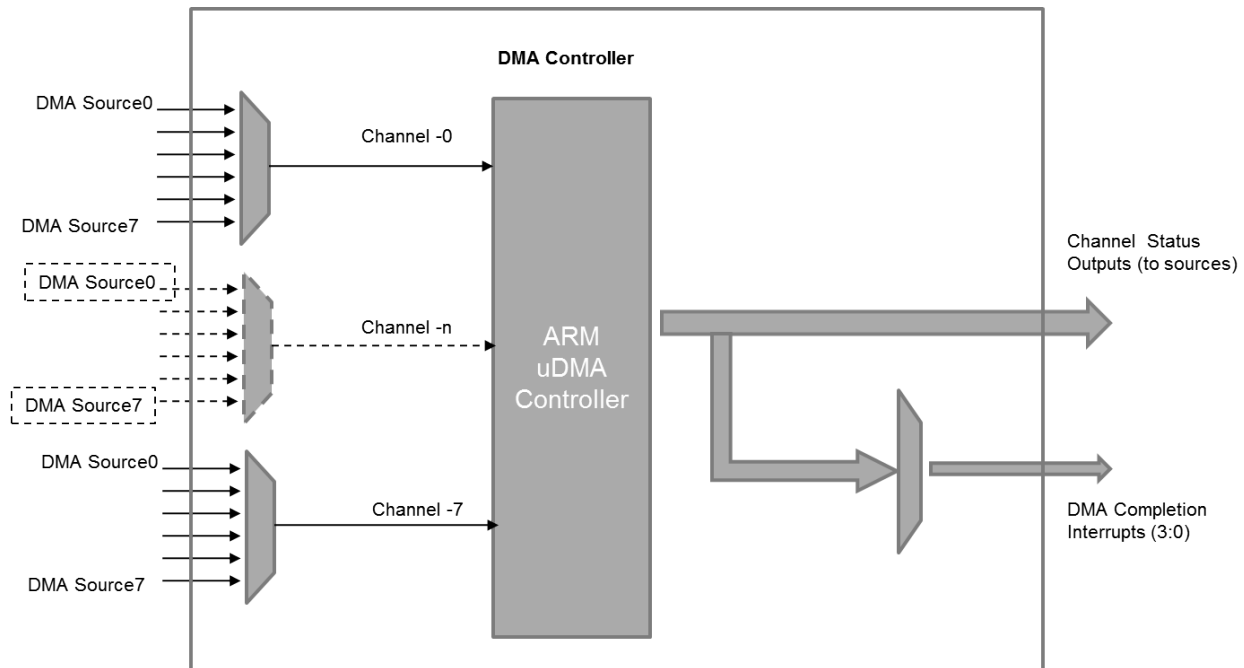
Figure 6-11. DMA Block Diagram
