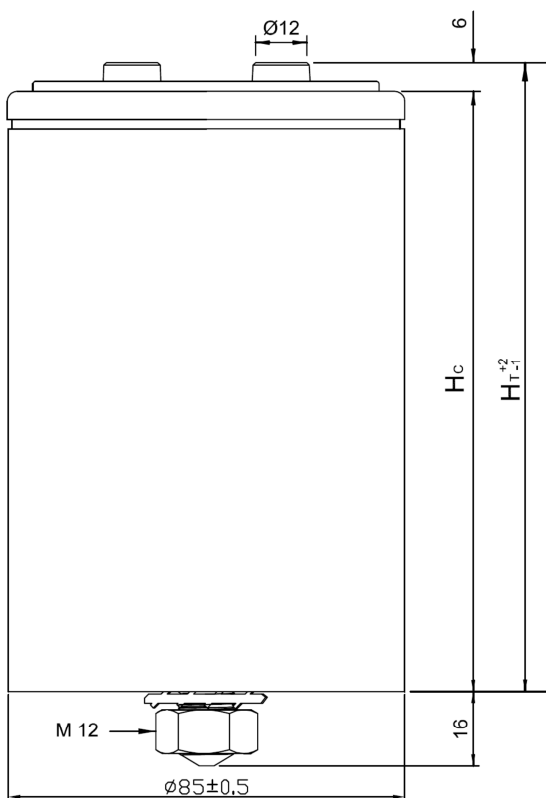
Figure 1: - B25620B - Ø 85mm - Female terminals (M6) - Between terminals 32\pm0.5 mm
