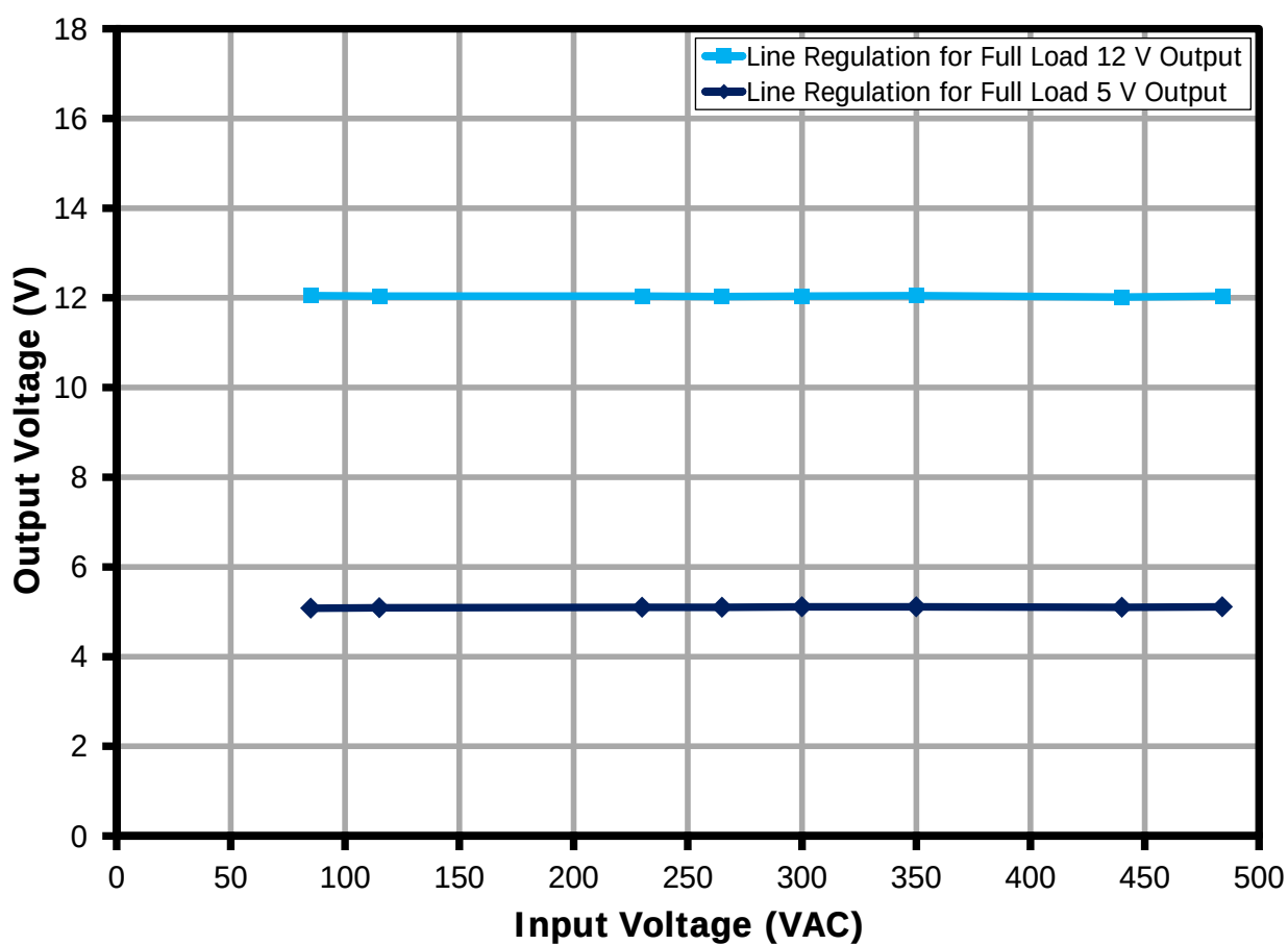
Figure 11 – Output Voltage vs. Input Line Voltage, Room Temperature.
