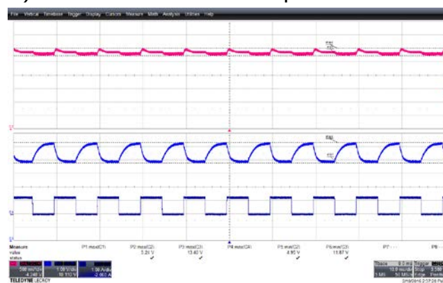
Figure 26 – 0.0 A – 1.25 A, 12 V Load Step Transient Response, 484 VAC.
