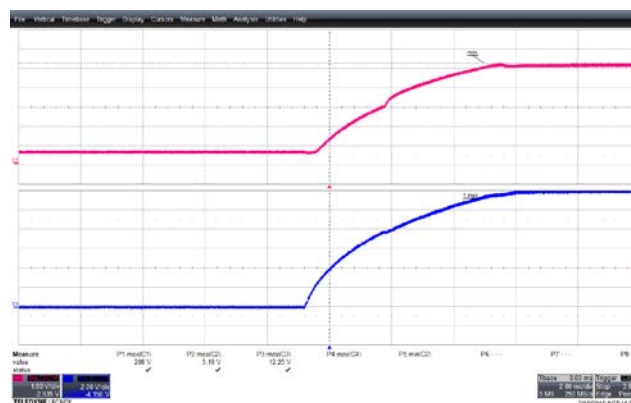
Figure 32 – Output Voltage Waveforms. 484 VAC Input. Upper: 5 V, 1 V / div. Lower: 12 V, 2 V / div., 2 ms / div.
