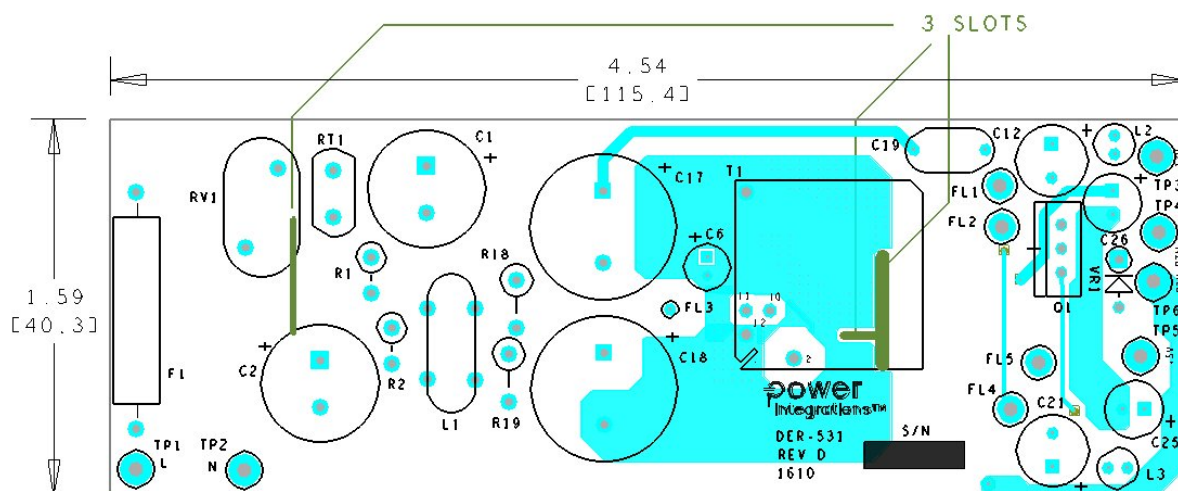
Figure 4 – Printed Circuit Layout, Top.
