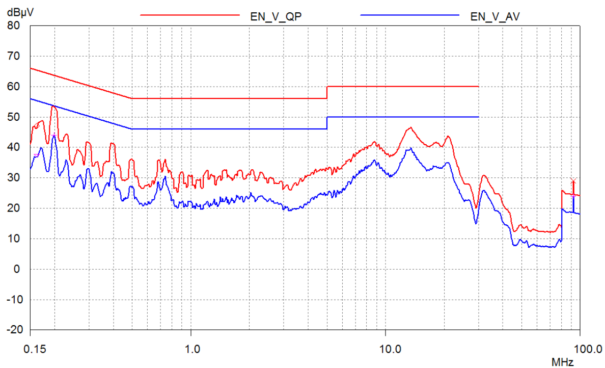
Figure 44 – Earth Ground at 110 VAC, Line.
