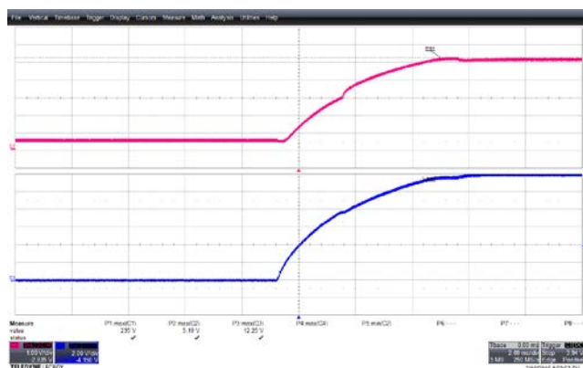
Figure 31 – Output Voltage Waveforms. 85 VAC Input. Upper: 5 V, 1 V / div. Lower: 12 V, 2 V / div, 2 ms / div.
