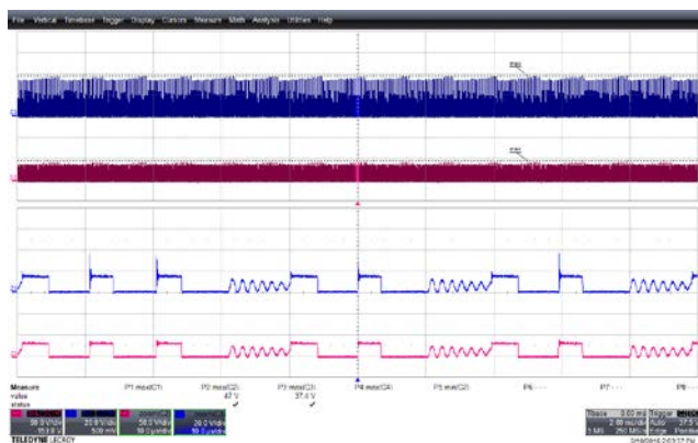
Figure 29 – SR FET Voltage Waveforms. 85 VAC Input, Full Load. Upper: 5 V, 20 V / , 2 ms, 10 \mu s / div. Lower: 12 V, 50 V / div.
