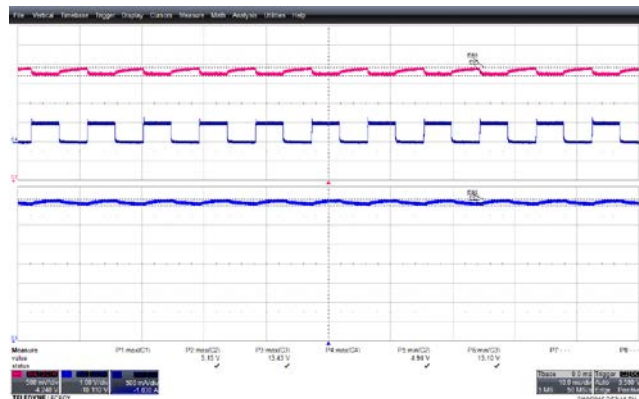
Figure 19 – 0.0 A – 0.5 A, 5 V Load Step Transient Response, 85 VAC. 5 V MIN : 4.94 V. 5 V MAX : 5.15 V. 12 V MIN : 13.10 V. 12 V MAX : 13.43 V. Upper: 5 V OUT , 0.5 V / div. Middle: 5 V Load, 0.5 A, 10 ms / div. Lower: 12 V OUT , 1 V / div.
