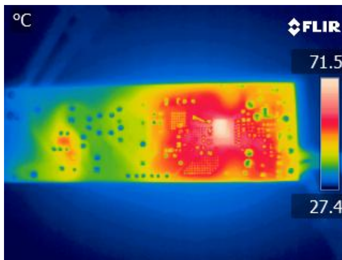
Figure 16 – InnoSwitch-EP Side. 85 VAC, Full Load.
