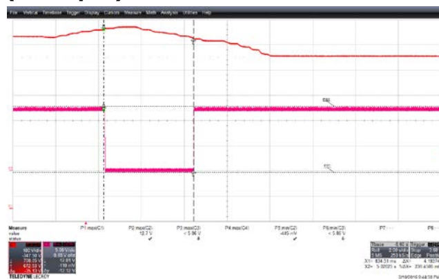
Figure 42 – Line Overvoltage.
