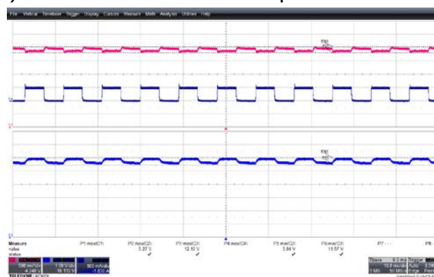
Figure 22 – 0.0 A – 0.5 A, 5 V Load Step Transient Response, 484 VAC. 5 V_{MIN} : 5.04 V. 5 V_{MAX} : 5.27 V. 12 V_{MIN} : 11.57 V. 12 V_{MAX} : 12.10 V. Upper: 5 V_{OUT} , 0.5 V / div. Middle: 5 V Load, 0.5 A, 10 ms / div. Lower: 12 V_{OUT} , 1 V / div.
