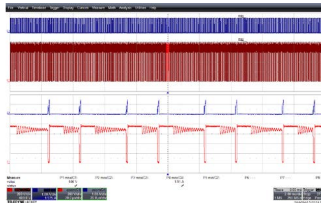
Figure 28 – Drain Voltage and Current Waveforms. 484 VAC Input, Full Load, (Max V_{DRAIN} : 806 V.) Upper: V_{DRAIN} , 200 V, 2 ms, 10 \mu s / div. Lower: I_{DRAIN} , 1000 mA / div.
