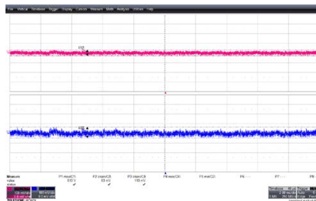
Figure 40 – Output Voltage Ripple Waveforms. 484 VAC Input. 1.25 A on 12 V. 5 V_{PK} : 63 mV, 12 V_{PK} : 113 mV. Upper: 5 V, 100 mV / div. Lower: 12 V, 100 mV, 2 ms / div..
