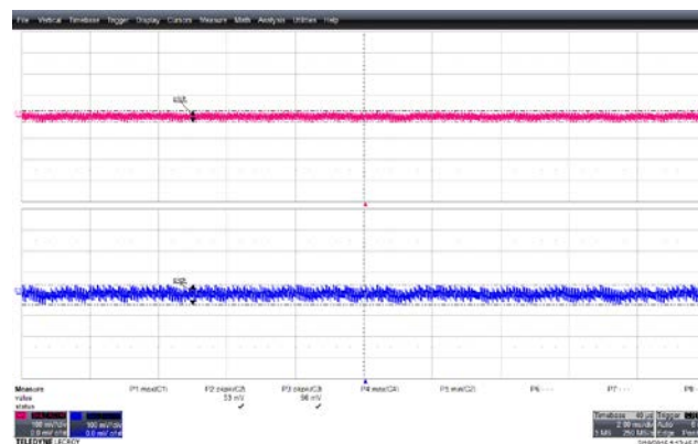
Figure 38 – Output Voltage Ripple Waveforms. 265 VAC Input. 1.25 A on 12 V. 5 V_{PK} : 53 mV, 12 V_{PK} : 96 mV. Upper: 5 V, 100 mV / div. Lower: 12 V, 100 mV, 2 ms / div.
