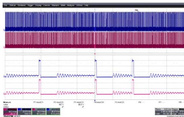
Figure 30 – SR FET Voltage Waveforms. 484 VAC Input, Full Load. (143 V MAX for 12 V, 66.6 V MAX for 5 V.) Upper: 5 V, 20 V / , 2 ms, 10 \mu s / div. Lower: 12 V, 50 V / div.
