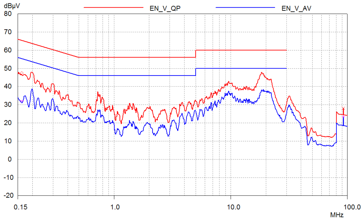
Figure 45 – Earth Ground at 230 VAC, Neutral.
