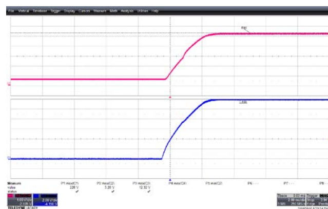
Figure 33 – Output Voltage Waveforms. 85 VAC Input. Upper: 5 V, 1 V / div. Lower: 12 V, 2 V / div., 2 ms / div.
