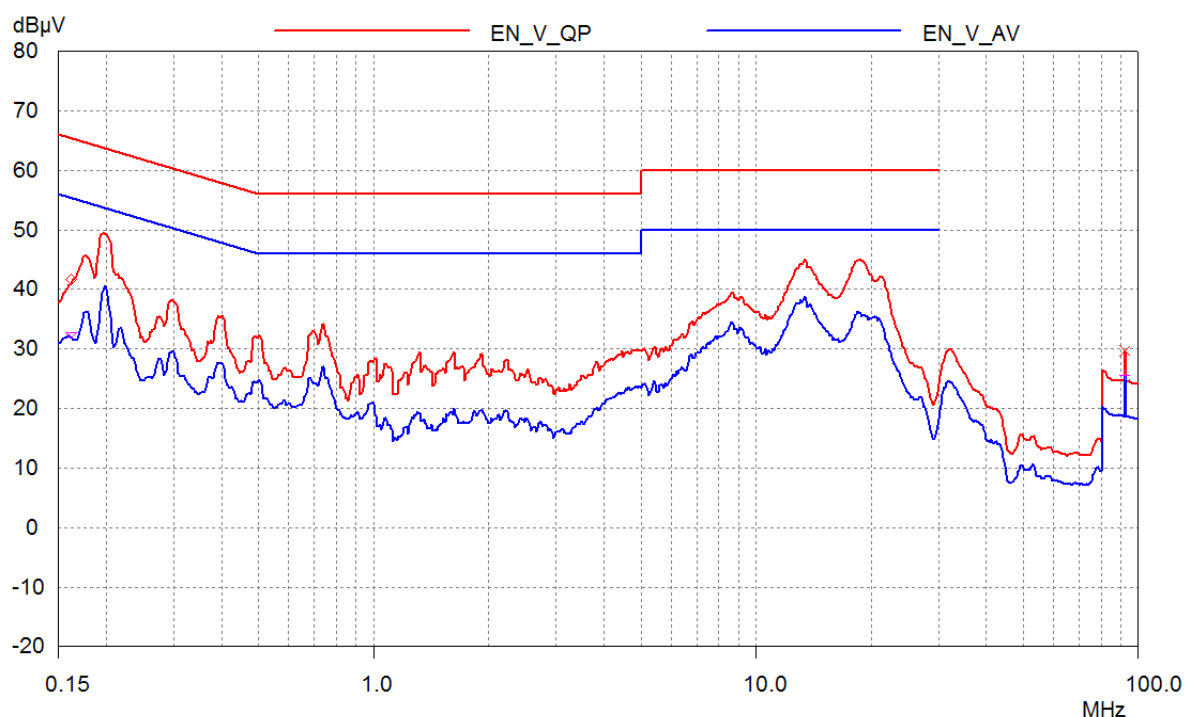
Figure 43 – Earth Ground at 110 VAC, Neutral.
