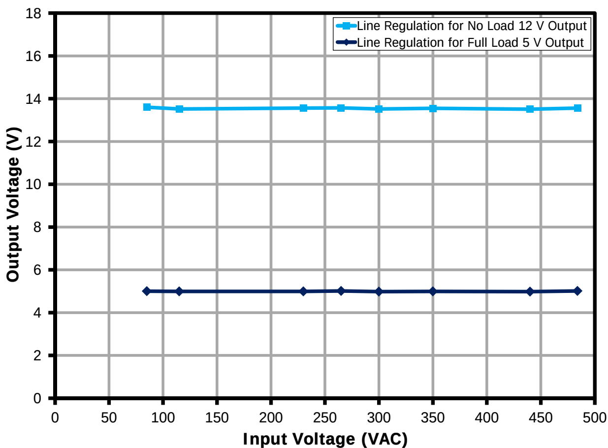
Figure 12 – 12 V Output Voltage vs. No Load, Room Temperature.
