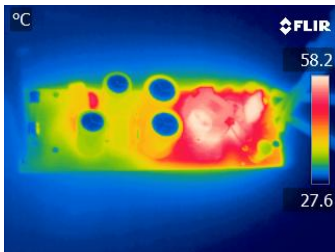
Figure 15 – Transformer Side. 85 VAC, Full Load.
