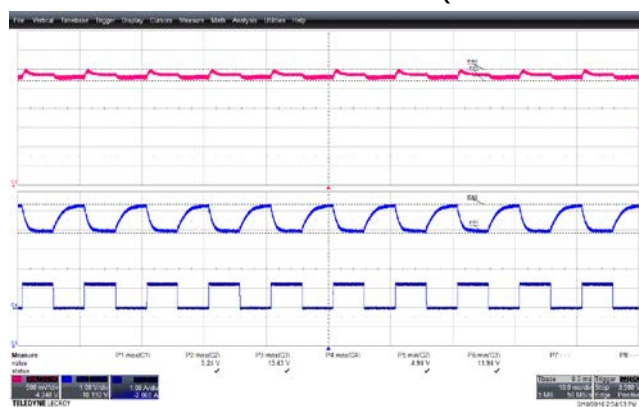
Figure 25 – 0.0 A – 1.25 A, 12 V Load Step Transient Response, 85 VAC.
