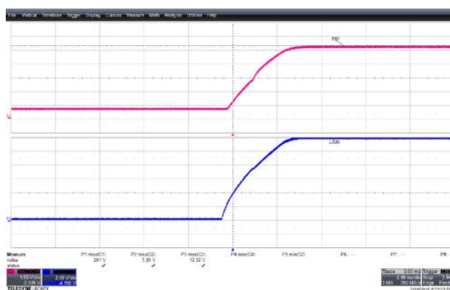
Figure 34 – Output Voltage Waveforms. 484 VAC Input. Upper: 5 V, 1 V / div. Lower: 12 V, 2 V / div., 2 ms / div.
