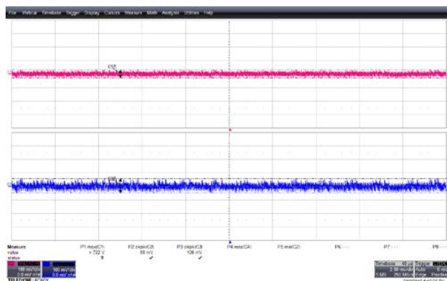
Figure 39 – Output Voltage Ripple Waveforms. 440 VAC Input. 1.25 A on 12 V. 5 V_{PK} : 60 mV, 12 V_{PK} : 106 mV. Upper: 5 V, 100 mV / div. Lower: 12 V, 100 mV, 2 ms / div.
