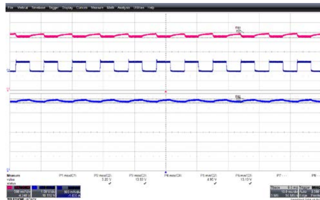
Figure 20 – 0.0 A – 0.5 A, 5 V Load Step Transient Response, 484 VAC. 5 V MIN : 4.95 V. 5 V MAX : 5.20 V. 12 V MIN : 13.13 V. 12 V MAX : 13.53 V. Upper: 5 V OUT , 0.5 V / div. Middle: 5 V Load, 0.5 A, 10 ms / div. Lower: 12 V OUT , 1 V / div.
