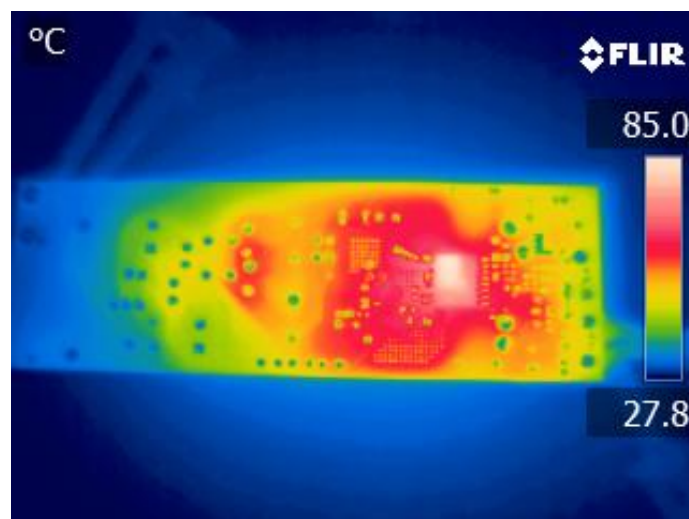
Figure 18 – InnoSwitch-EP Side. 265 VAC, Full Load.
