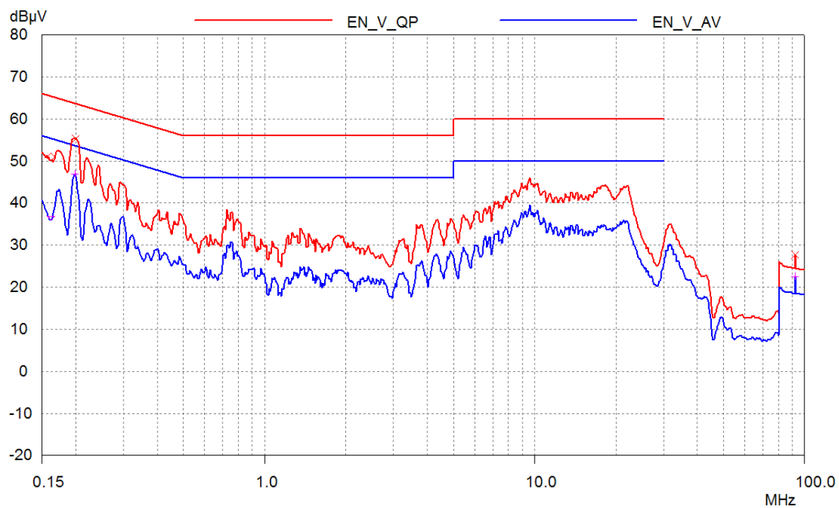
Figure 46 – Earth Ground at 230 VAC, Line.
