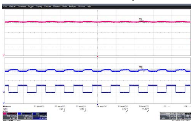
Figure 23 – 0.0 A – 1.25 A, 12 V Load Step Transient Response, 85 VAC. 5 V_{MIN} : 5.10 V. 5 V_{MAX} : 5.24 V. 12 V_{MIN} : 11.64 V. 12 V_{MAX} : 12.07 V. Upper: 5 V_{OUT} , 0.5 V / div. Middle: 12 V_{OUT} , 1 V / div. Lower: 12 V Load, 1 A, 10 ms / div.
