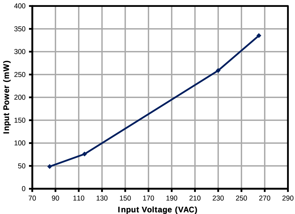
Figure 10 – No-Load Input Power vs. Input Line Voltage, Room Temperature.
