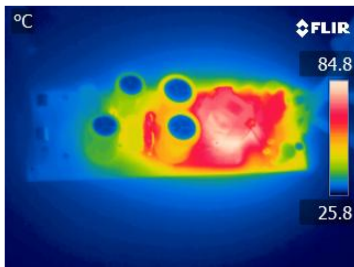
Figure 17 – Transformer Side. 265 VAC, Full Load.
