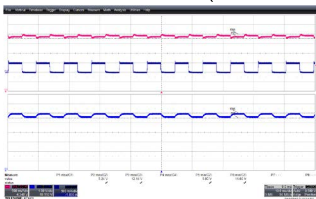
Figure 21 – 0.0 A – 0.5 A, 5 V Load Step Transient Response, 85 VAC. 5 V_{MIN} : 5.00 V. 5 V_{MAX} : 5.24 V. 12 V_{MIN} : 11.60 V. 12 V_{MAX} : 12.14 V. Upper: 5 V_{OUT} , 0.5 V / div. Middle: 5 V Load, 0.5 A, 10 ms / div. Lower: 12 V_{OUT} , 1 V / div.
