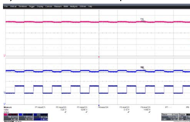
Figure 24 – 0.0 A – 1.25 A, 12 V Load Step Transient Response, 484 VAC. 5 V_{MIN} : 5.10 V. 5 V_{MAX} : 5.24 V. 12 V_{MIN} : 11.60 V. 12 V_{MAX} : 12.04 V. Upper: 5 V_{OUT} , 0.5 V / div. Middle: 12 V_{OUT} , 1 V / div. Lower: 12 V Load, 1 A, 10 ms / div.
