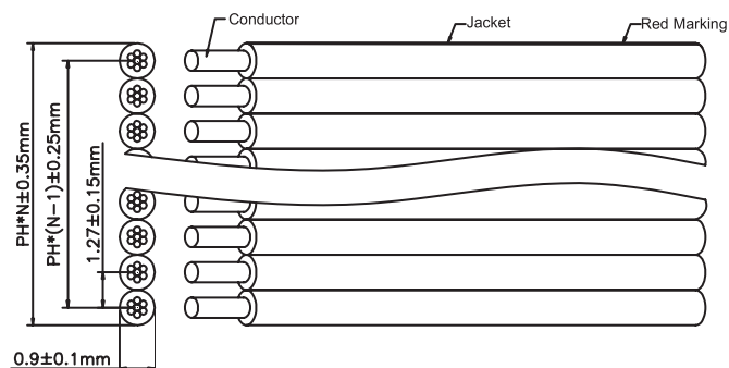
Structural View
