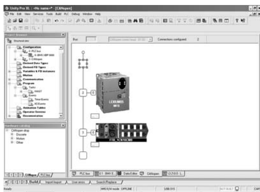
Example of Unity™ Pro configuration screen for Lexium® 05 servo drive and Modicon® FTB IP 67 I/O splitter box
