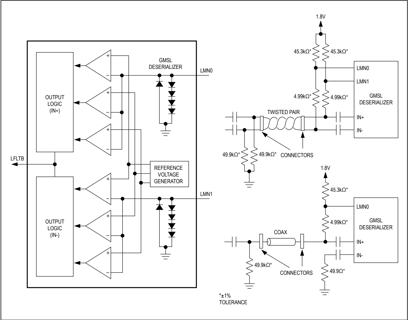
Figure 4. Line Fault
